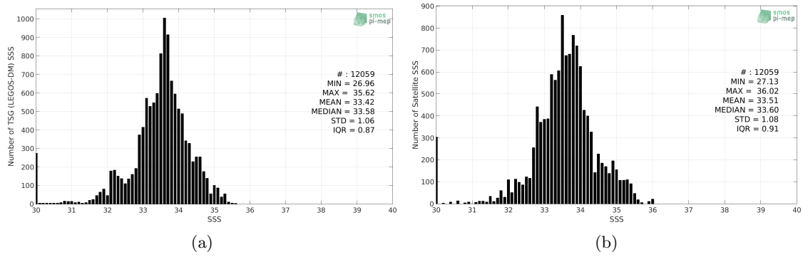
Figure 2: Histograms of SSS from TSG (LEGOS-DM) (a) and SMOS SSS L3 v4 - 9 Days (CATDS-CECOS-LOCEAN) (b) considering all match-up pairs per bins of 0.1 over the Ganga and Brahmaputra river plumes Pi-MEP region and for the full satellite product period.
