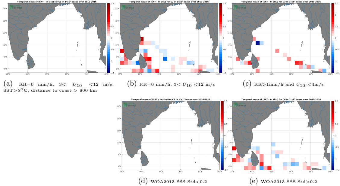
Figure 12: Temporal mean gridded over spatial boxes of size 1^{\circ}\times 1^{\circ} of \Delta\text{SSS} (SMOS SSS L3 v4 - 9 Days (CATDS-CECOS-LOCEAN) - TSG (LEGOS-DM)) for 5 different subdatasets corresponding to: RR=0 mm/h, 3 < U_{10} < 12 m/s, SST >5^{\circ}\text{C} , distance to coast > 800 km (a), RR=0 mm/h, 3 < U_{10} < 12 m/s (b), RR >1 mm/h and U_{10} < 4 m/s (c), WOA2013 SSS Std <0.2 (d), WOA2013 SSS Std >0.2 (e).
