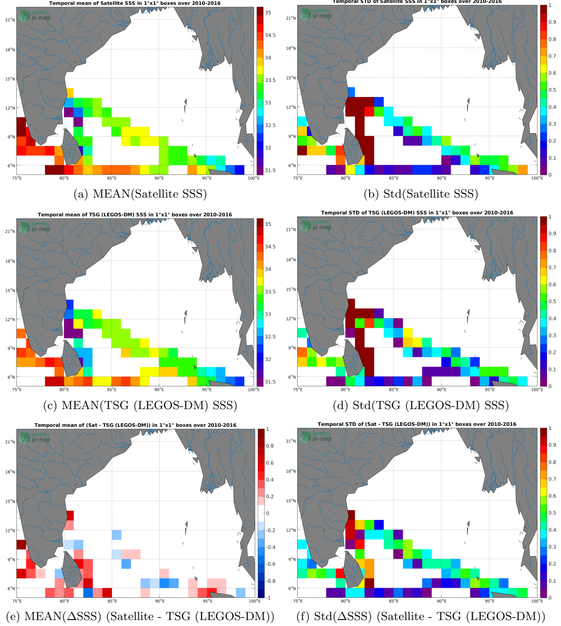
Figure 6: Temporal mean (left) and Std (right) of SSS from SMOS SSS L3 v4 - 9 Days (CATDS-CECOS-LOCEAN) (top), TSG (LEGOS-DM) (middle), and of \Delta SSS (Satellite - TSG (LEGOS-DM)). Only match-up pairs are used to generate these maps.
