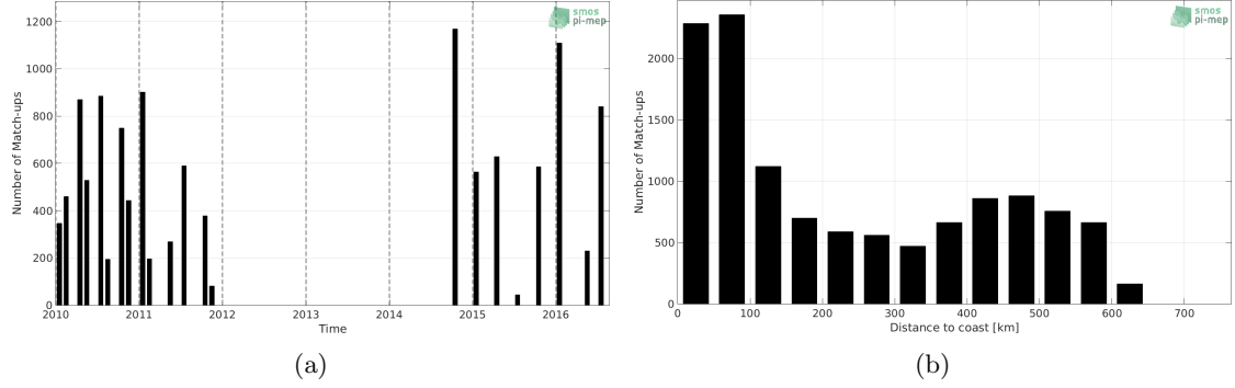
Figure 1: Number of match-ups between TSG (LEGOS-DM) and SMOS SSS L3 v4 - 9 Days (CATDS-CECOS-LOCEAN) SSS as a function of time (a) and as function of the distance to coast (b) over the Ganga and Brahmaputra river plumes Pi-MEP region and for the full satellite product period.
