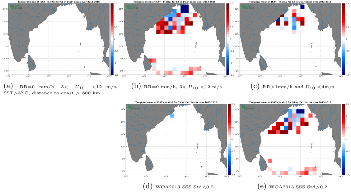
Figure 11: Temporal mean gridded over spatial boxes of size 1^{\circ}\times 1^{\circ} of \Delta\text{SSS} (SMOS SSS L3 v4 - 9 Days (CATDS-CECOS-LOCEAN) - Surface drifters) for 5 different subdatasets corresponding to: RR=0 mm/h, 3 < U_{10} < 12 m/s, SST >5^{\circ}\text{C} , distance to coast > 800 km (a), RR=0 mm/h, 3 < U_{10} < 12 m/s (b), RR >1 mm/h and U_{10} < 4 m/s (c), WOA2013 SSS Std <0.2 (d), WOA2013 SSS Std >0.2 (e).
