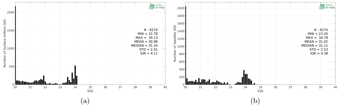
Figure 2: Histograms of SSS from Surface drifters (a) and SMOS SSS L3 v4 - 9 Days (CATDS-CECOS-LOCEAN) (b) considering all match-up pairs per bins of 0.1 over the Ganga and Brahmaputra river plumes Pi-MEP region and for the full satellite product period.
