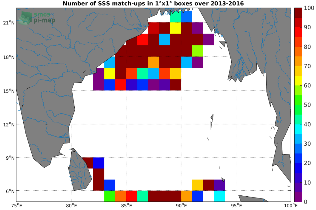
Figure 3: Number of SSS match-ups between Surface drifters SSS and the SMOS SSS L3 v4 - 9 Days (CATDS-CECOS-LOCEAN) SSS product for the Ganga and Brahmaputra river plumes Pi-MEP region over 1^\circ \times 1^\circ boxes and for the full satellite product period.
