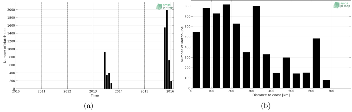
Figure 1: Number of match-ups between Surface drifters and SMOS SSS L3 v4 - 9 Days (CATDS-CECOS-LOCEAN) SSS as a function of time (a) and as function of the distance to coast (b) over the Ganga and Brahmaputra river plumes Pi-MEP region and for the full satellite product period.
