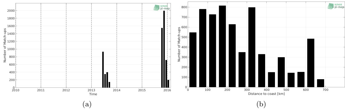
Figure 1: Number of match-ups between Surface drifters and SMOS-L3-CATDS-CECOS-LOCEAN-V4-9DAYS-25KM SSS as a function of time (a) and as function of the distance to coast (b) over the Ganga and Brahmaputra river plumes Pi-MEP region and for the full satellite product period.
