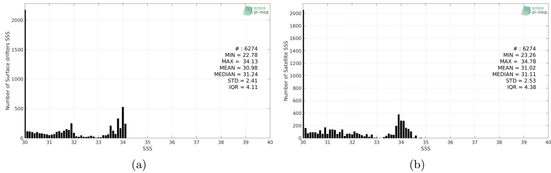
Figure 2: Histograms of SSS from Surface drifters (a) and SMOS-L3-CATDS-CECOS-LOCEAN-V4-9DAYS-25KM (b) considering all match-up pairs per bins of 0.1 over the Ganga and Brahmaputra river plumes Pi-MEP region and for the full satellite product period.
