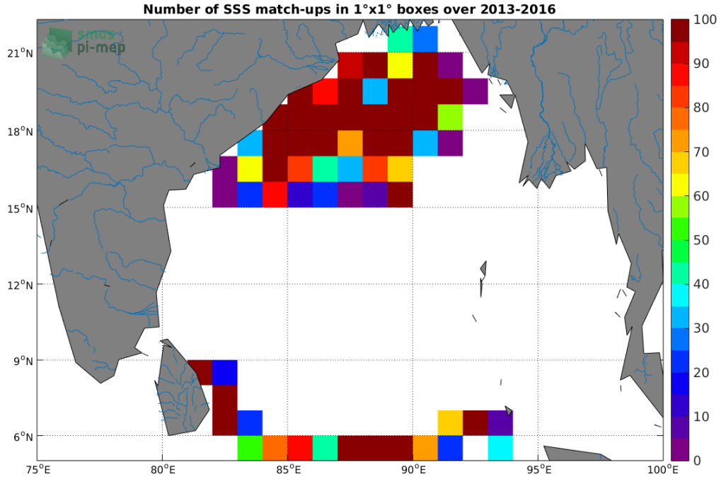
Figure 3: Number of SSS match-ups between Surface drifters SSS and the SMOS-L3-CATDS-CECOS-LOCEAN-V4-9DAYS-25KM SSS product for the Ganga and Brahmaputra river plumes Pi-MEP region over 1^\circ \times 1^\circ boxes and for the full satellite product period.
