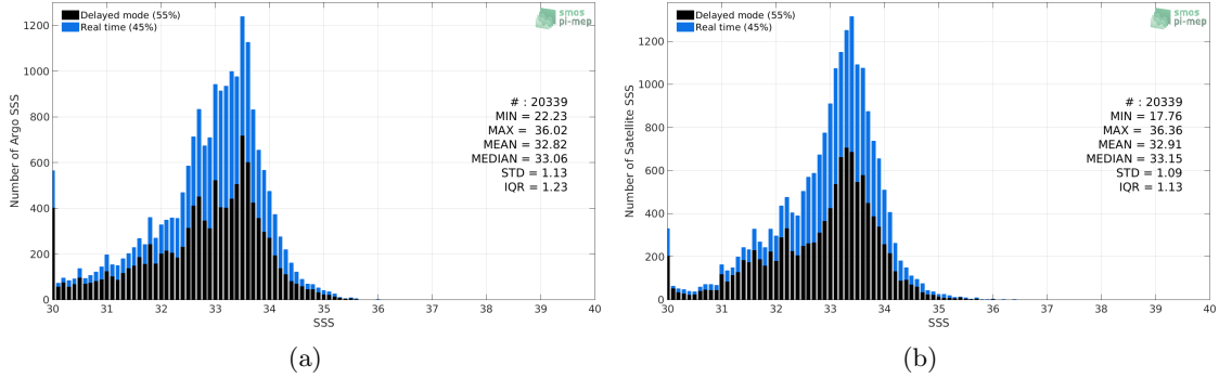
Figure 2: Histograms of SSS from Argo (a) and SMOS SSS L3 v4 - 18 Days (CATDS-CECOS-LOCEAN) (b) considering all match-up pairs per bins of 0.1 over the Ganga and Brahmaputra river plumes Pi-MEP region and for the full satellite product period.
