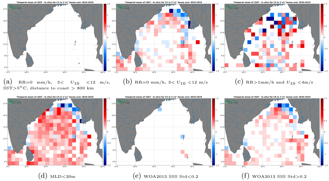
Figure 12: Temporal mean gridded over spatial boxes of size 1^\circ \times 1^\circ of \Delta SSS (SMOS SSS L3 v4 - 18 Days (CATDS-CECOS-LOCEAN) - Argo) for 6 different subdatasets corresponding to: RR=0 mm/h, 3 < U_{10} < 12 m/s, SST > 5^\circ C , distance to coast > 800 km (a), RR=0 mm/h, 3 < U_{10} < 12 m/s (b), RR > 1 mm/h and U_{10} < 4 m/s (c), MLD < 20 m (d), WOA2013 SSS Std < 0.2 (e), WOA2013 SSS Std > 0.2 (f).
