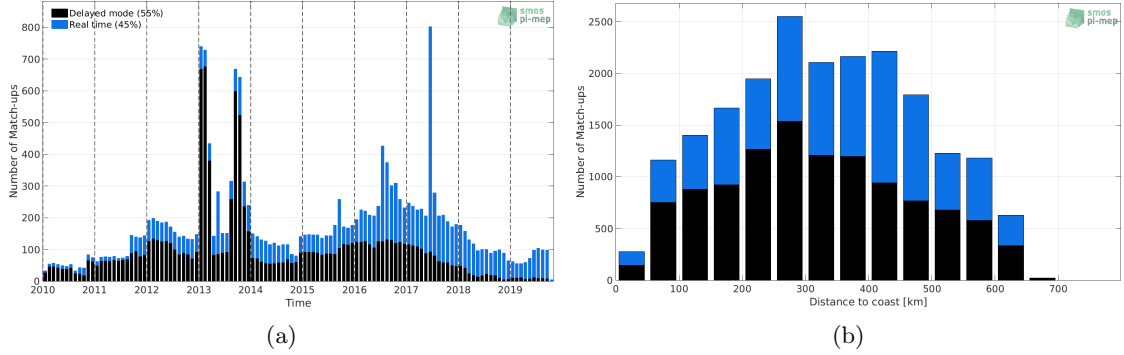
Figure 1: Number of match-ups between Argo and SMOS SSS L3 v4 - 18 Days (CATDS-CECOS-LOCEAN) SSS as a function of time (a) and as function of the distance to coast (b) over the Ganga and Brahmaputra river plumes Pi-MEP region and for the full satellite product period.
