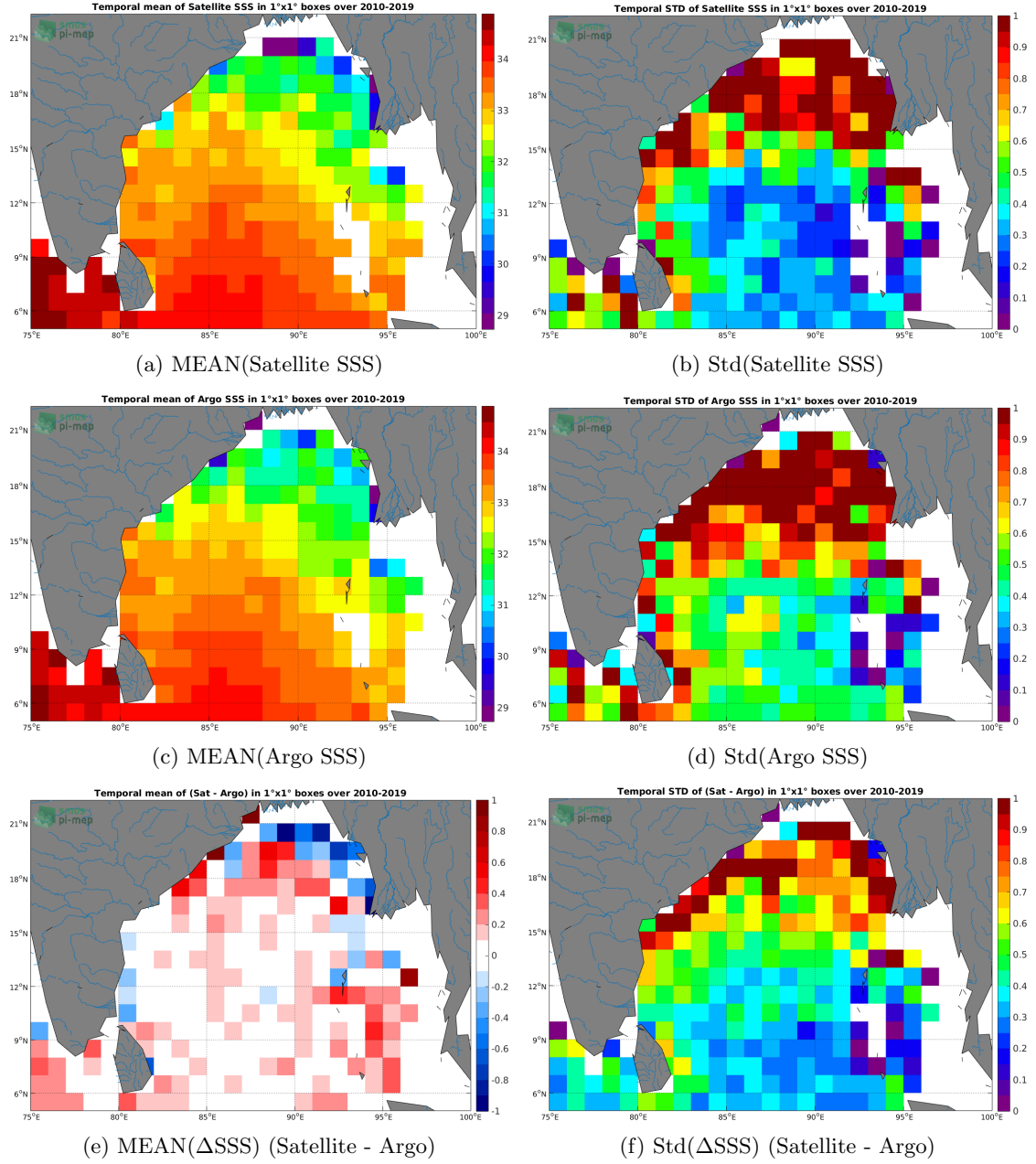
Figure 6: Temporal mean (left) and Std (right) of SSS from SMOS SSS L3 v4 - 18 Days (CATDS-CECOS-LOCEAN) (top), Argo (middle), and of \Delta SSS (Satellite - Argo). Only match-up pairs are used to generate these maps.
