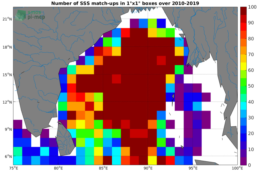
Figure 4: Number of SSS match-ups between Argo SSS and the SMOS SSS L3 v4 - 18 Days (CATDS-CECOS-LOCEAN) SSS product for the Ganga and Brahmaputra river plumes Pi-MEP region over 1°x1° boxes and for the full satellite product period.
