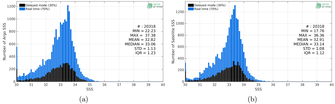
Figure 2: Histograms of SSS from Argo (a) and SMOS-L3-CATDS-CECOS-LOCEAN-V4-18DAYS-25KM (b) considering all match-up pairs per bins of 0.1 over the Ganga and Brahmaputra river plumes Pi-MEP region and for the full satellite product period.
