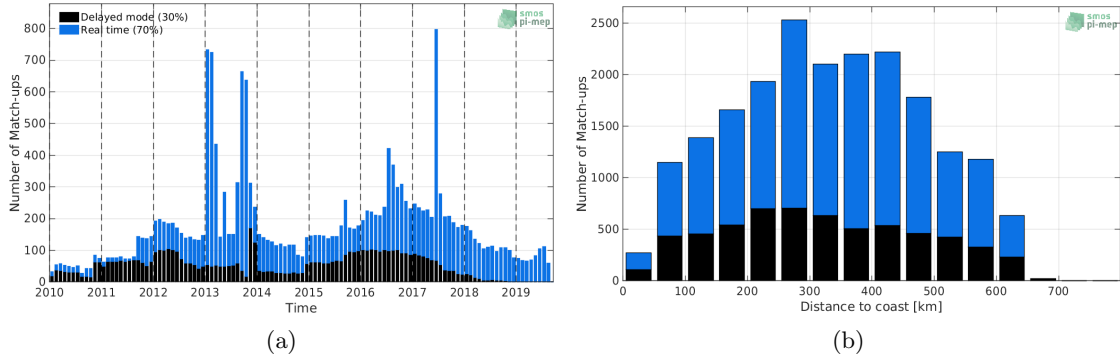
Figure 1: Number of match-ups between Argo and SMOS-L3-CATDS-CECOS-LOCEAN-V4-18DAYS-25KM SSS as a function of time (a) and as function of the distance to coast (b) over the Ganga and Brahmaputra river plumes Pi-MEP region and for the full satellite product period.
