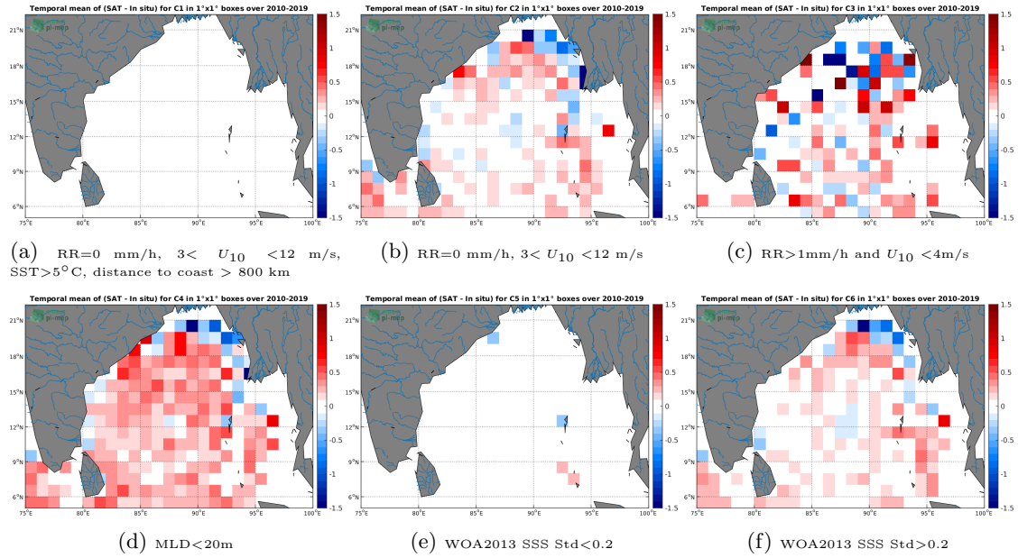
Figure 12: Temporal mean gridded over spatial boxes of size 1^\circ \times 1^\circ of \Delta SSS (SMOS-L3-CATDS-CECOS-LOCEAN-V4-18DAYS-25KM - Argo) for 6 different subdatasets corresponding to:RR=0 mm/h, 3 < U_{10} < 12 m/s, SST >5^\circ C, distance to coast > 800 km (a), RR=0 mm/h, 3 < U_{10} < 12 m/s (b), RR >1 mm/h and U_{10} < 4 m/s (c),MLD <20 m (d),WOA2013 SSS Std <0.2 (e),WOA2013 SSS Std >0.2 (f).
