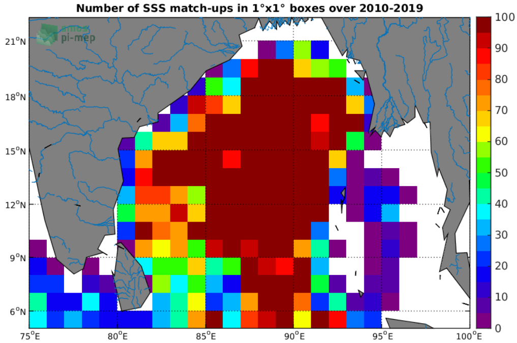
Figure 4: Number of SSS match-ups between Argo SSS and the SMOS-L3-CATDS-CECOS-LOCEAN-V4-18DAYS-25KM SSS product for the Ganga and Brahmaputra river plumes Pi-MEP region over 1°x1° boxes and for the full satellite product period.
