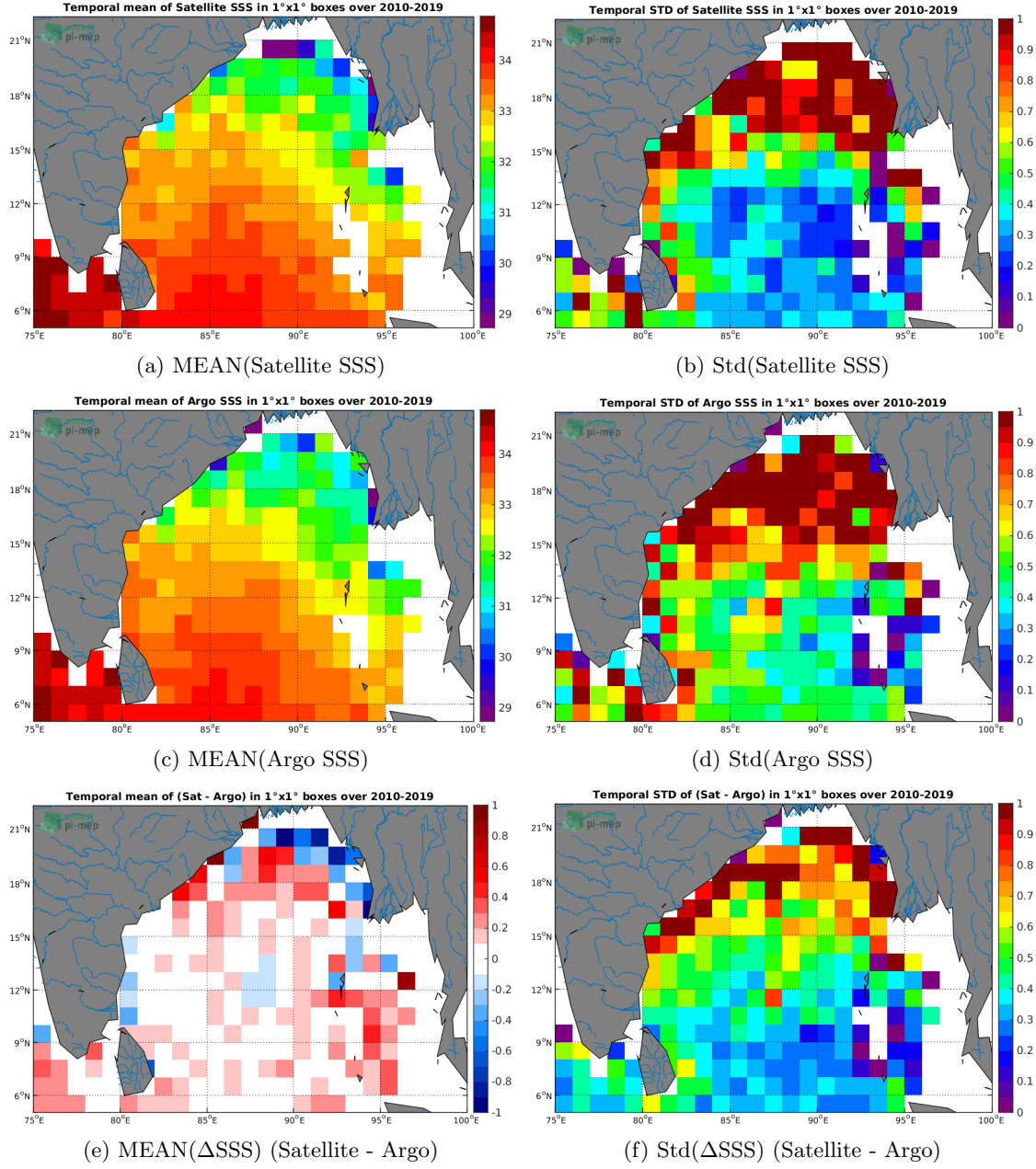
Figure 6: Temporal mean (left) and Std (right) of SSS from SMOS-L3-CATDS-CECOS-LOCEAN-V4-18DAYS-25KM (top), Argo (middle), and of \Delta SSS (Satellite - Argo). Only match-up pairs are used to generate these maps.
