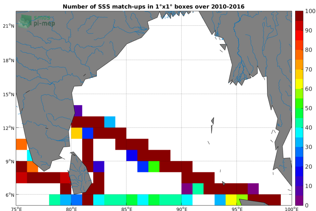
Figure 4: Number of SSS match-ups between TSG-LEGOS-DM SSS and the SMOS-L3-CATDS-CECOS-LOCEAN-V3-9DAYS-25KM SSS product for the Ganga and Brahmaputra river plumes Pi-MEP region over 1^\circ \times 1^\circ boxes and for the full satellite product period.
