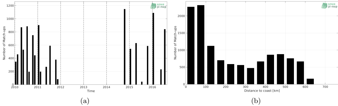
Figure 1: Number of match-ups between TSG-LEGOS-DM and SMOS-L3-CATDS-CECOS-LOCEAN-V3-9DAYS-25KM SSS as a function of time (a) and as function of the distance to coast (b) over the Ganga and Brahmaputra river plumes Pi-MEP region and for the full satellite product period.
