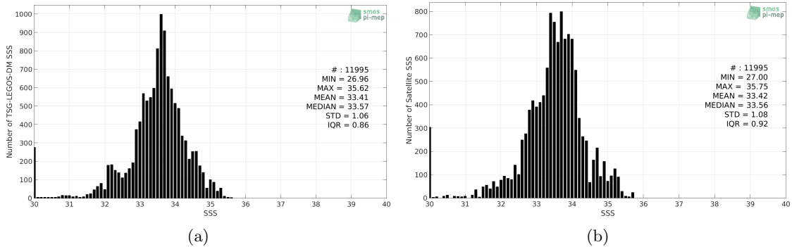
Figure 2: Histograms of SSS from TSG-LEGOS-DM (a) and SMOS-L3-CATDS-CECOS-LOCEAN-V3-9DAYS-25KM (b) considering all match-up pairs per bins of 0.1 over the Ganga and Brahmaputra river plumes Pi-MEP region and for the full satellite product period.
