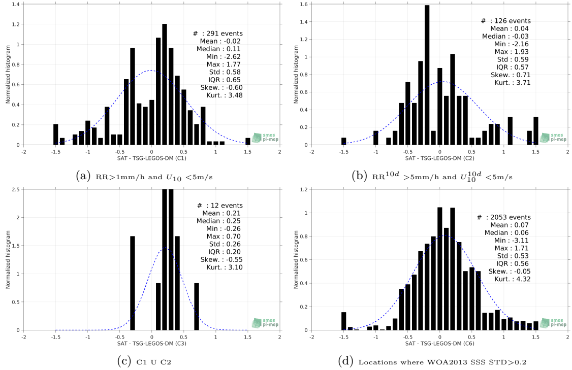
Figure 13: Normalized histogram of \Delta SSS (SMOS-L3-CATDS-CECOS-LOCEAN-V3-9DAYS-25KM - TSG-LEGOS-DM) for 6 different subdatasets corresponding to: RR > 1mm/h and U_{10} < 5 m/s (a), RR 10d > 5mm/h and U_{10}^{10d} < 5 m/s (b), C1 U C2 (c), Locations where WOA2013 SSS STD > 0.2 (d).
