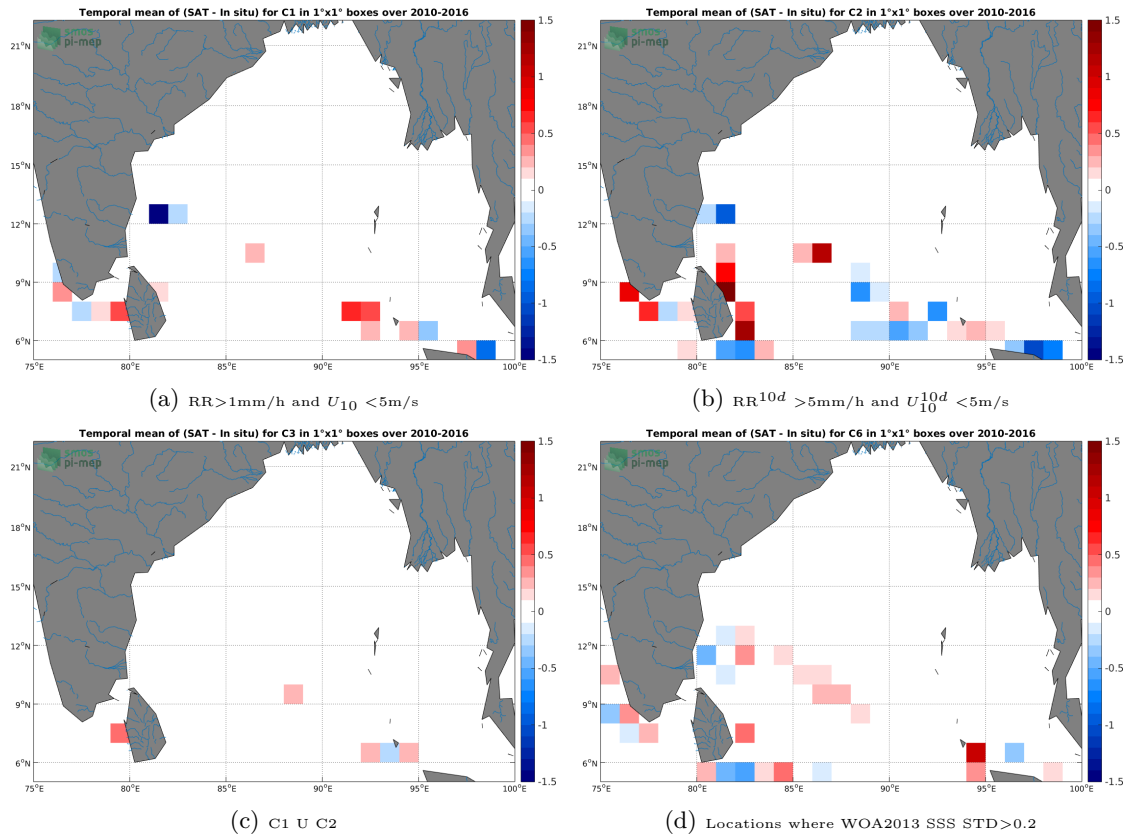
Figure 12: Temporal mean gridded over spatial boxes of size 1^\circ \times 1^\circ of \Delta SSS (SMOS-L3-CATDS-CECOS-LOCEAN-V3-9DAYS-25KM - TSG-LEGOS-DM) for 4 different subdatasets corresponding to: RR > 1mm/h and U_{10} < 5\text{m/s} (a), RR^{10d} > 5\text{mm/h} and U_{10}^{10d} < 5\text{m/s} (b), C1 U C2 (c), Locations where WOA2013 SSS STD > 0.2 (d).
