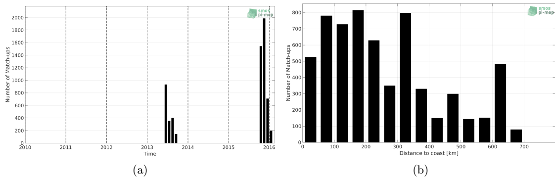
Figure 1: Number of match-ups between Surface drifters and SMOS-L3-CATDS-CECOS-LOCEAN-V3-9DAYS-25KM SSS as a function of time (a) and as function of the distance to coast (b) over the Ganga and Brahmaputra river plumes Pi-MEP region and for the full satellite product period.
