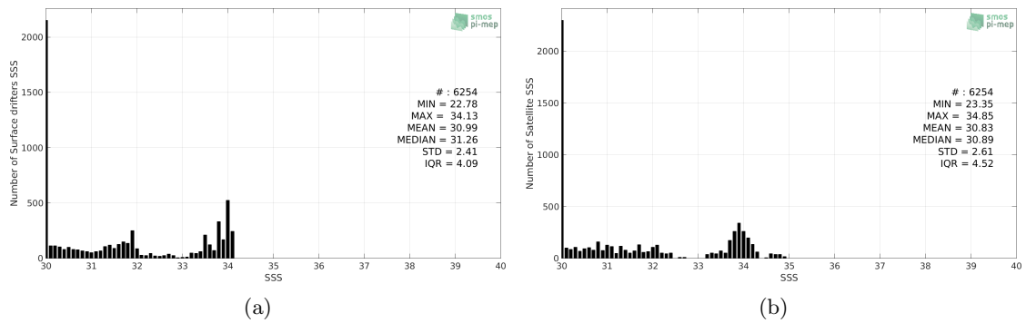
Figure 2: Histograms of SSS from Surface drifters (a) and SMOS-L3-CATDS-CECOS-LOCEAN-V3-9DAYS-25KM (b) considering all match-up pairs per bins of 0.1 over the Ganga and Brahmaputra river plumes Pi-MEP region and for the full satellite product period.
