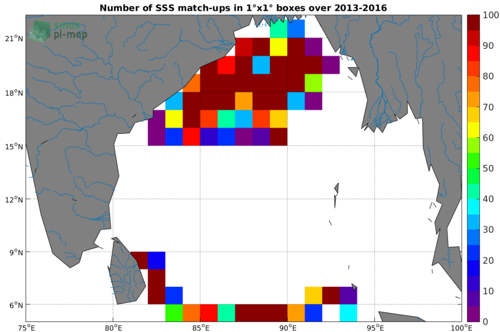
Figure 3: Number of SSS match-ups between Surface drifters SSS and the SMOS-L3-CATDS-CECOS-LOCEAN-V3-9DAYS-25KM SSS product for the Ganga and Brahmaputra river plumes Pi-MEP region over 1°x1° boxes and for the full satellite product period.
