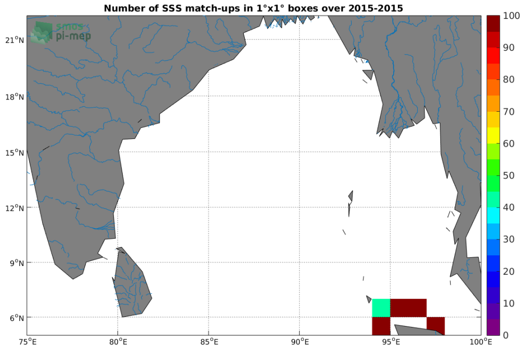
Figure 4: Number of SSS match-ups between TSG-SAMOS SSS and the SMOS-L3-CATDS-CECOS-LOCEAN-V3-18DAYS-25KM SSS product for the Ganga and Brahmaputra river plumes Pi-MEP region over 1^\circ \times 1^\circ boxes and for the full satellite product period.
