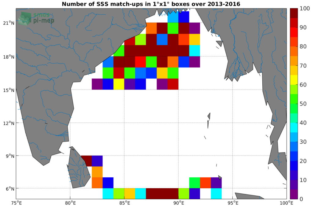
Figure 3: Number of SSS match-ups between Surface drifters SSS and the SMOS-L3-CATDS-CECOS-LOCEAN-V3-18DAYS-25KM SSS product for the Ganga and Brahmaputra river plumes Pi-MEP region over 1^\circ \times 1^\circ boxes and for the full satellite product period.
