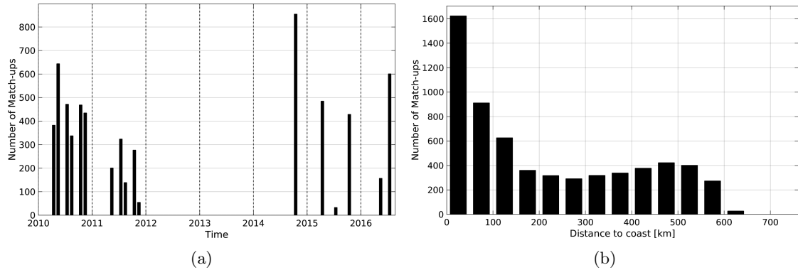
Figure 1: Number of match-ups between TSG-LEGOS-DM and SMOS-L3-CATDS-CECOS-LOCEAN-V2-9DAYS-25KM SSS as a function of time (a) and as function of the distance to coast (b) over the Ganga and Brahmaputra river plumes Pi-MEP region and for the full satellite product period.
