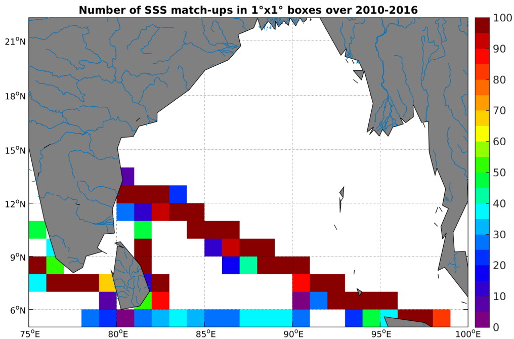
Figure 4: Number of SSS match-ups between TSG-LEGOS-DM SSS and the SMOS-L3-CATDS-CECOS-LOCEAN-V2-9DAYS-25KM SSS product for the Ganga and Brahmaputra river plumes Pi-MEP region over 1°x1° boxes and for the full satellite product period.
