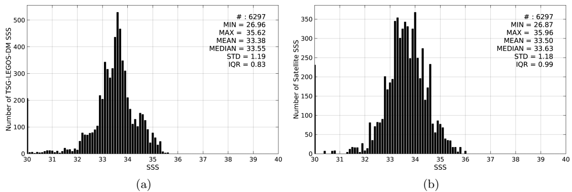
Figure 2: Histograms of SSS from TSG-LEGOS-DM (a) and SMOS-L3-CATDS-CECOS-LOCEAN-V2-9DAYS-25KM (b) considering all match-up pairs per bins of 0.1 over the Ganga and Brahmaputra river plumes Pi-MEP region and for the full satellite product period.
