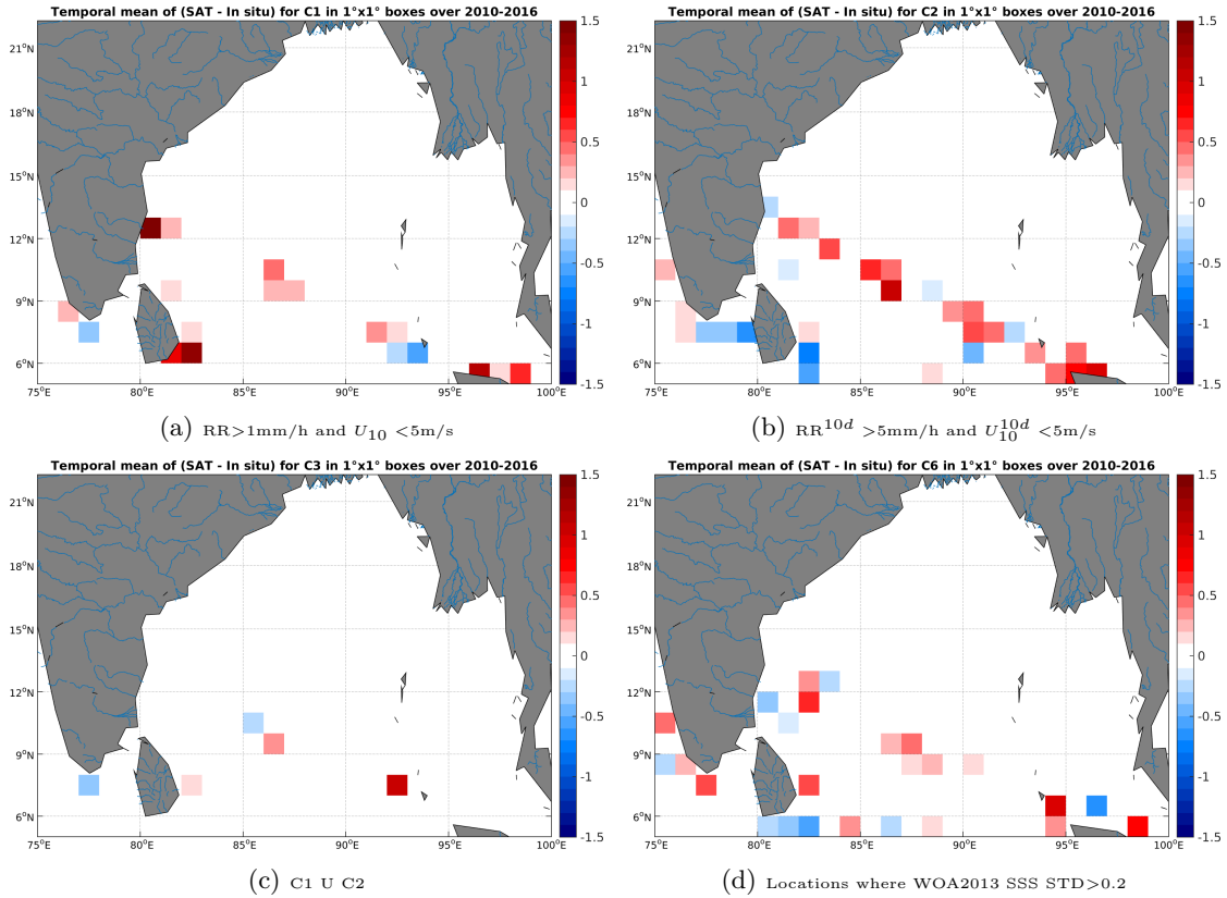
Figure 12: Temporal mean gridded over spatial boxes of size 1°x1° of \Delta SSS (SMOS-L3-CATDS-CECOS-LOCEAN-V2-9DAYS-25KM - TSG-LEGOS-DM) for 4 different subdatasets corresponding to:RR>1mm/h and U_{10} < 5 m/s (a), RR^{10d} > 5 mm/h and U_{10}^{10d} < 5 m/s (b), C1 U C2 (c),Locations where WOA2013 SSS STD>0.2 (d).
