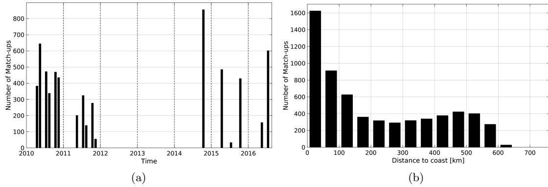
Figure 1: Number of match-ups between TSG-LEGOS-DM and SMOS-L3-CATDS-CECOS-LOCEAN-V2-9DAYS-25KM SSS as a function of time (a) and as function of the distance to coast (b) over the Ganga and Brahmaputra river plumes Pi-MEP region and for the full satellite product period.
