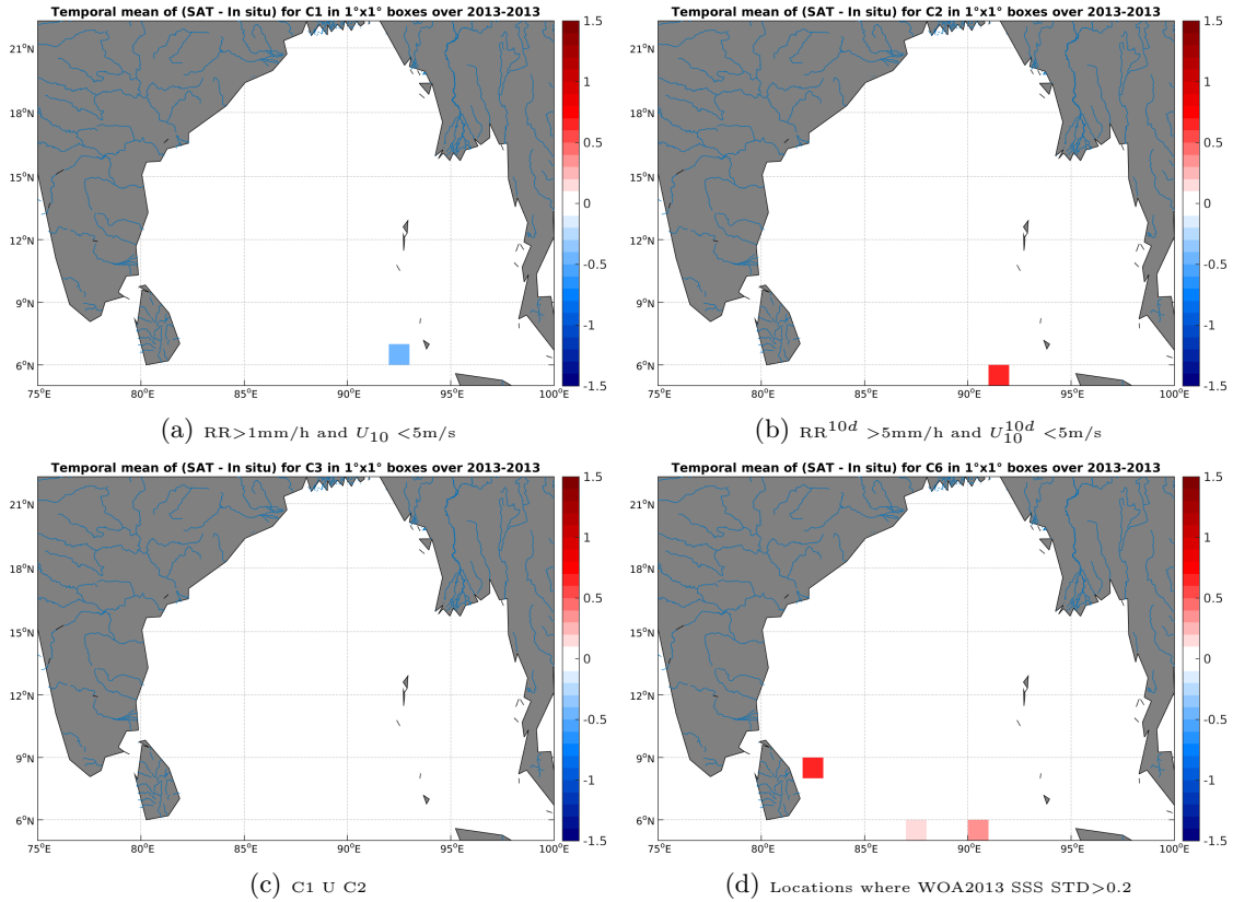
Figure 11: Temporal mean gridded over spatial boxes of size 1°x1° of \Delta SSS (SMOS-L3-CATDS-CECOS-LOCEAN-V2-9DAYS-25KM - Surface drifters) for 4 different subdatasets corresponding to: RR > 1\text{mm/h} and U_{10} < 5\text{m/s} (a), RR^{10d} > 5\text{mm/h} and U_{10}^{10d} < 5\text{m/s} (b), C1 U C2 (c), Locations where WOA2013 SSS STD > 0.2 (d).
