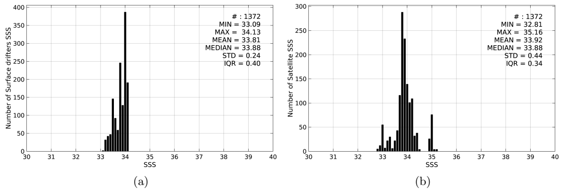
Figure 2: Histograms of SSS from Surface drifters (a) and SMOS-L3-CATDS-CECOS-LOCEAN-V2-9DAYS-25KM (b) considering all match-up pairs per bins of 0.1 over the Ganga and Brahmaputra river plumes Pi-MEP region and for the full satellite product period.
