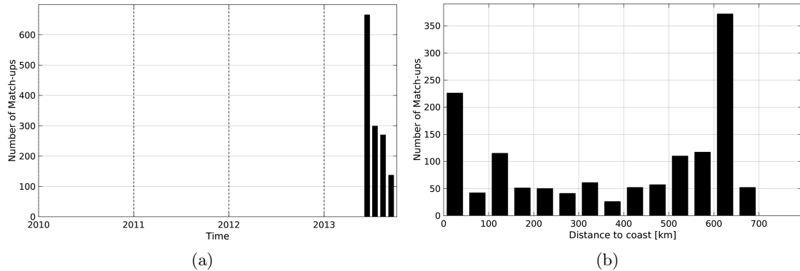
Figure 1: Number of match-ups between Surface drifters and SMOS-L3-CATDS-CECOS-LOCEAN-V2-9DAYS-25KM SSS as a function of time (a) and as function of the distance to coast (b) over the Ganga and Brahmaputra river plumes Pi-MEP region and for the full satellite product period.
