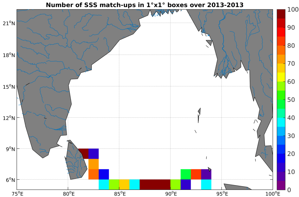
Figure 3: Number of SSS match-ups between Surface drifters SSS and the SMOS-L3-CATDS-CECOS-LOCEAN-V2-9DAYS-25KM SSS product for the Ganga and Brahmaputra river plumes Pi-MEP region over 1^{\circ} \times 1^{\circ} boxes and for the full satellite product period.
