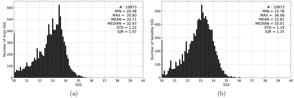
Figure 2: Histograms of SSS from Argo (a) and SMOS-L3-CATDS-CECOS-LOCEAN-V2-9DAYS-25KM (b) considering all match-up pairs per bins of 0.1 over the Ganga and Brahmaputra river plumes Pi-MEP region and for the full satellite product period.
