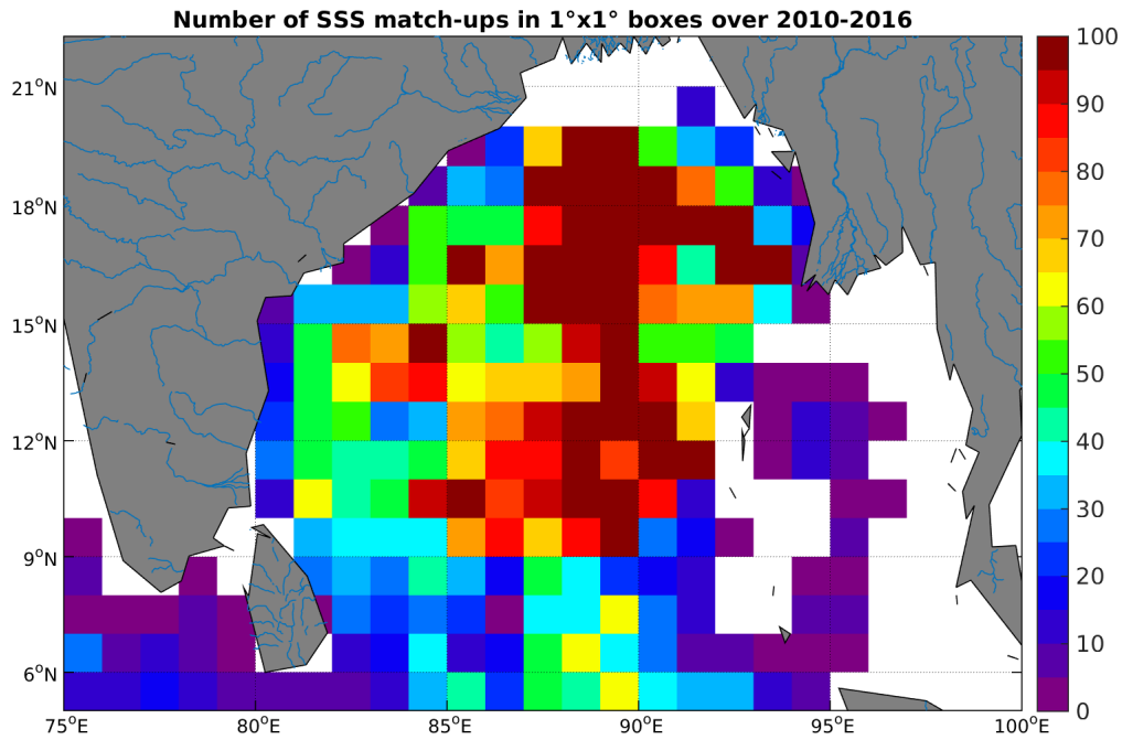
Figure 4: Number of SSS match-ups between Argo SSS and the SMOS-L3-CATDS-CECOS-LOCEAN-V2-9DAYS-25KM SSS product for the Ganga and Brahmaputra river plumes Pi-MEP region over 1°x1° boxes and for the full satellite product period.
