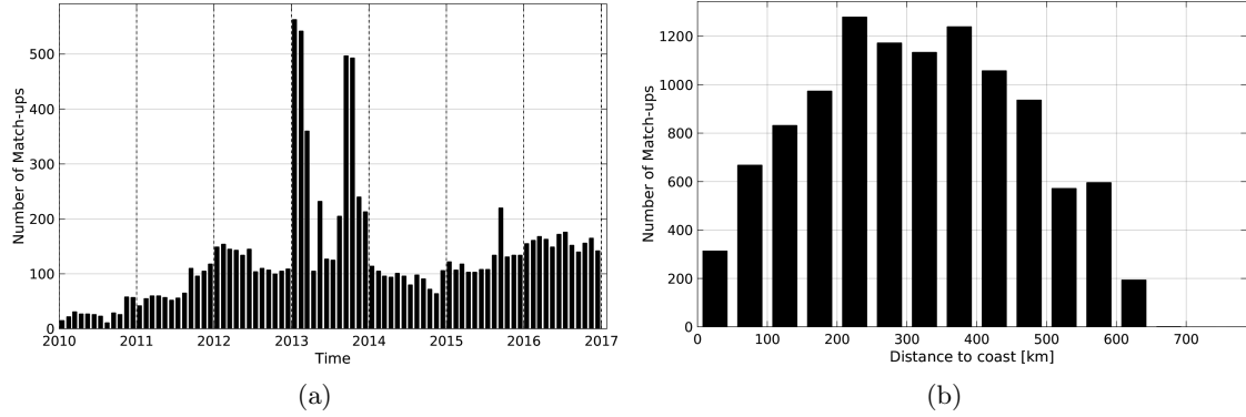
Figure 1: Number of match-ups between Argo and SMOS-L3-CATDS-CECOS-LOCEAN-V2-9DAYS-25KM SSS as a function of time (a) and as function of the distance to coast (b) over the Ganga and Brahmaputra river plumes Pi-MEP region and for the full satellite product period.
