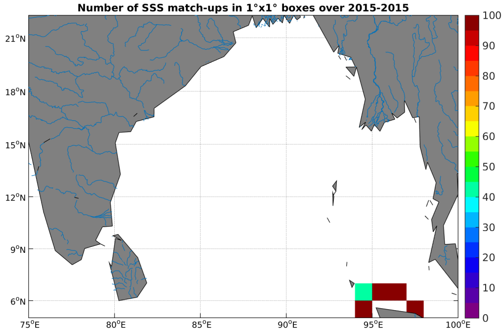
Figure 4: Number of SSS match-ups between TSG-SAMOS SSS and the SMOS-L3-CATDS-CECOS-LOCEAN-V2-18DAYS-25KM SSS product for the Ganga and Brahmaputra river plumes Pi-MEP region over 1^\circ \times 1^\circ boxes and for the full satellite product period.
