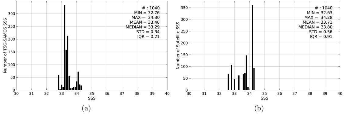
Figure 2: Histograms of SSS from TSG-SAMOS (a) and SMOS-L3-CATDS-CECOS-LOCEAN-V2-18DAYS-25KM (b) considering all match-up pairs per bins of 0.1 over the Ganga and Brahmaputra river plumes Pi-MEP region and for the full satellite product period.
