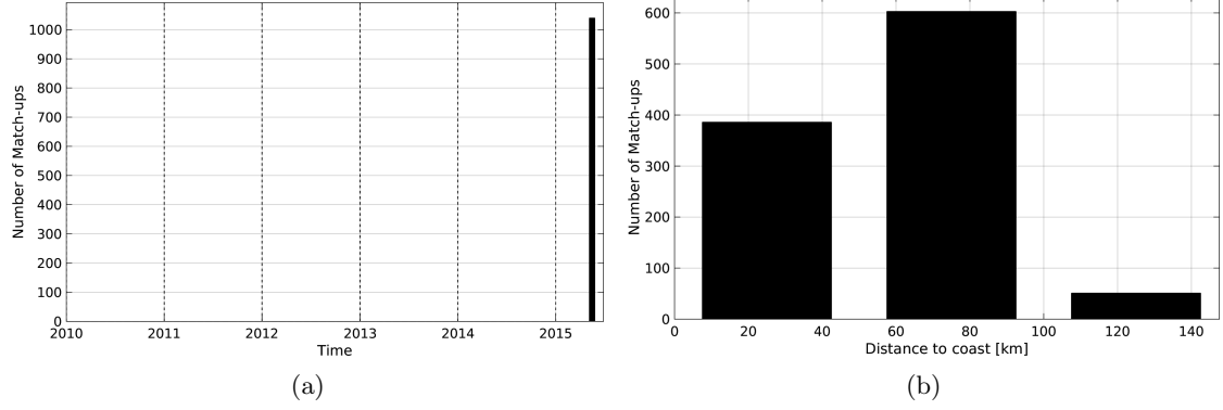
Figure 1: Number of match-ups between TSG-SAMOS and SMOS-L3-CATDS-CECOS-LOCEAN-V2-18DAYS-25KM SSS as a function of time (a) and as function of the distance to coast (b) over the Ganga and Brahmaputra river plumes Pi-MEP region and for the full satellite product period.
