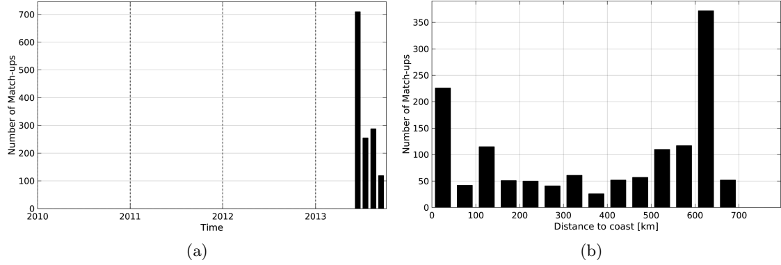
Figure 1: Number of match-ups between Surface drifters and SMOS-L3-CATDS-CECOS-LOCEAN-V2-18DAYS-25KM SSS as a function of time (a) and as function of the distance to coast (b) over the Ganga and Brahmaputra river plumes Pi-MEP region and for the full satellite product period.
