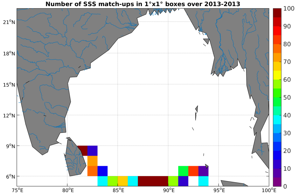
Figure 3: Number of SSS match-ups between Surface drifters SSS and the SMOS-L3-CATDS-CECOS-LOCEAN-V2-18DAYS-25KM SSS product for the Ganga and Brahmaputra river plumes Pi-MEP region over 1^\circ \times 1^\circ boxes and for the full satellite product period.
