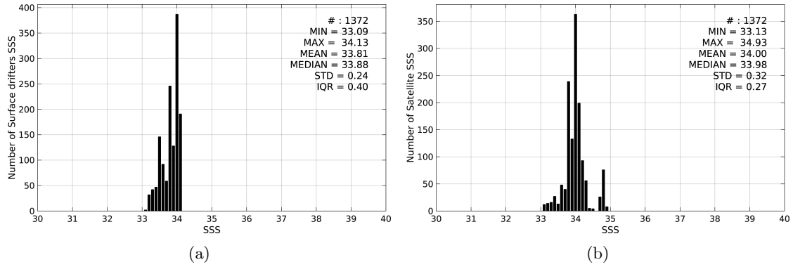
Figure 2: Histograms of SSS from Surface drifters (a) and SMOS-L3-CATDS-CECOS-LOCEAN-V2-18DAYS-25KM (b) considering all match-up pairs per bins of 0.1 over the Ganga and Brahmaputra river plumes Pi-MEP region and for the full satellite product period.
