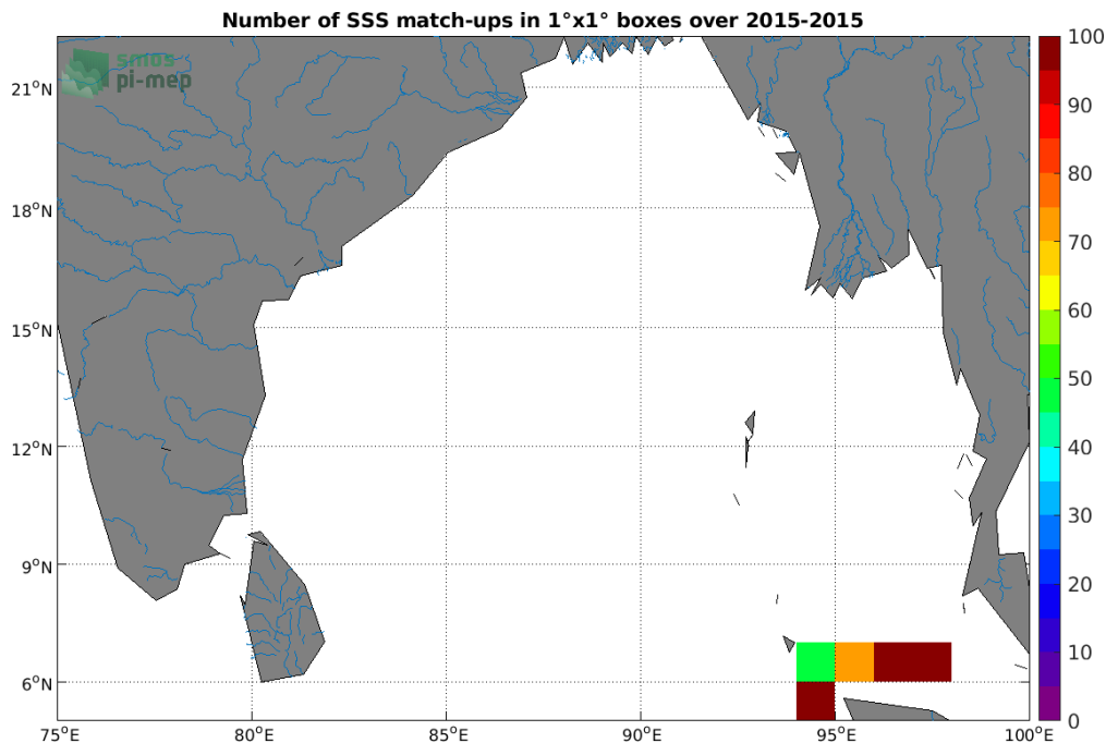
Figure 4: Number of SSS match-ups between TSG (SAMOS) SSS and the SMOS SSS L3 v2 - Monthly - 0.25 Deg (CATDS-CECOS-IFREMER) SSS product for the Ganga and Brahmaputra river plumes Pi-MEP region over 1^\circ \times 1^\circ boxes and for the full satellite product period.
