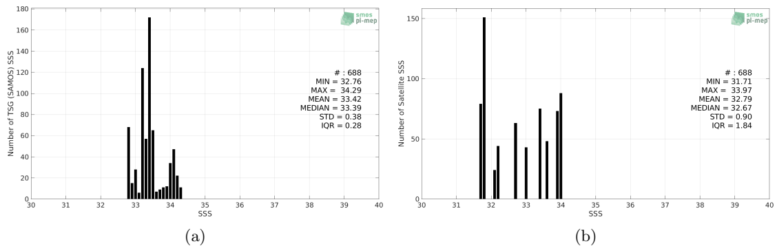
Figure 2: Histograms of SSS from TSG (SAMOS) (a) and SMOS SSS L3 v2 - Monthly - 0.25 Deg (CATDS-CECOS-IFREMER) (b) considering all match-up pairs per bins of 0.1 over the Ganga and Brahmaputra river plumes Pi-MEP region and for the full satellite product period.
