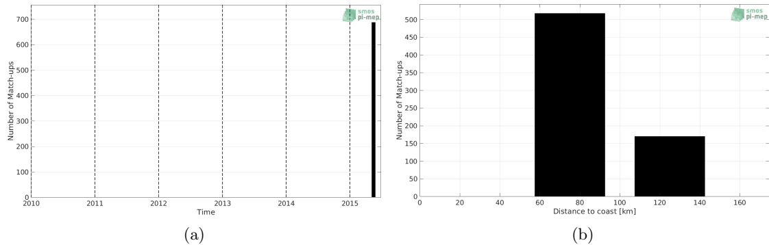
Figure 1: Number of match-ups between TSG (SAMOS) and SMOS SSS L3 v2 - Monthly - 0.25 Deg (CATDS-CECOS-IFREMER) SSS as a function of time (a) and as function of the distance to coast (b) over the Ganga and Brahmaputra river plumes Pi-MEP region and for the full satellite product period.
