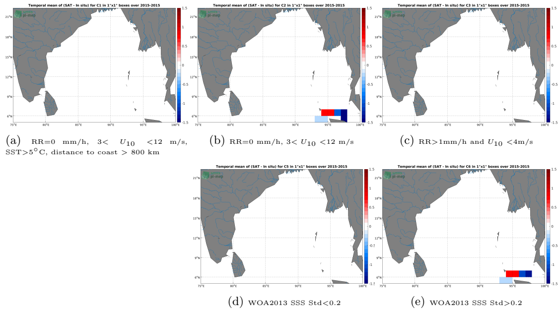
Figure 12: Temporal mean gridded over spatial boxes of size 1^{\circ}\times 1^{\circ} of \Delta\text{SSS} (SMOS SSS L3 v2 - Monthly - 0.25 Deg (CATDS-CECOS-IFREMER) - TSG (SAMOS)) for 5 different subdatasets corresponding to:RR=0 mm/h, 3 < U_{10} < 12 m/s, SST >5^{\circ}\text{C} , distance to coast > 800 km (a), RR=0 mm/h, 3 < U_{10} < 12 m/s (b), RR >1 mm/h and U_{10} < 4 m/s (c), WOA2013 SSS Std <0.2 (d), WOA2013 SSS Std >0.2 (e).
