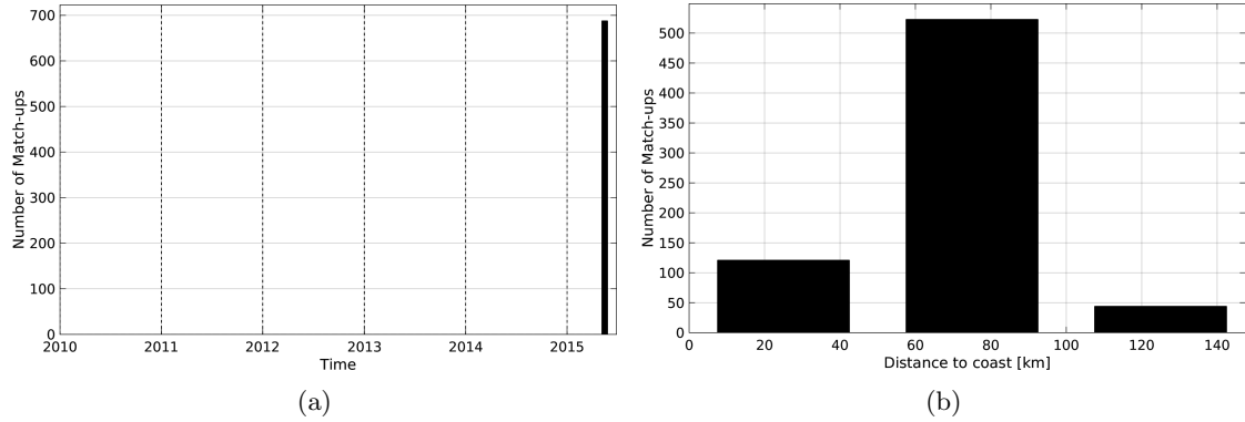
Figure 1: Number of match-ups between TSG-SAMOS and SMOS-L3-CATDS-IFREMER-CECOS-V2-MONTHLY-0.25DEG SSS as a function of time (a) and as function of the distance to coast (b) over the Ganga and Brahmaputra river plumes Pi-MEP region and for the full satellite product period.
