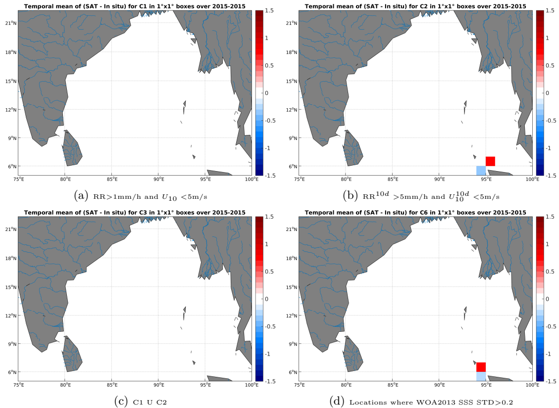
Figure 12: Temporal mean gridded over spatial boxes of size 1°x1° of \Delta SSS (SMOS-L3-CATDS-IFREMER-CECOS-V2-MONTHLY-0.25DEG - TSG-SAMOS) for 4 different subdatasets corresponding to:RR>1mm/h and U_{10} < 5\text{m/s} (a), RR^{10d} > 5\text{mm/h} and U_{10}^{10d} < 5\text{m/s} (b), C1 U C2 (c),Locations where WOA2013 SSS STD>0.2 (d).
