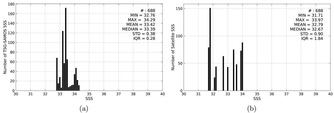
Figure 2: Histograms of SSS from TSG-SAMOS (a) and SMOS-L3-CATDS-IFREMER-CECOS-V2-MONTHLY-0.25DEG (b) considering all match-up pairs per bins of 0.1 over the Ganga and Brahmaputra river plumes Pi-MEP region and for the full satellite product period.
