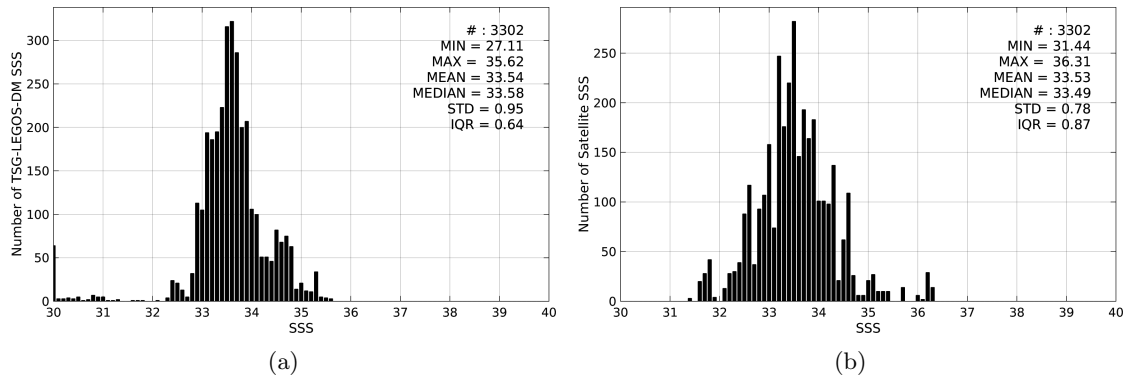
Figure 2: Histograms of SSS from TSG-LEGOS-DM (a) and SMOS-L3-CATDS-IFREMER-CECOS-V2-MONTHLY-0.25DEG (b) considering all match-up pairs per bins of 0.1 over the Ganga and Brahmaputra river plumes Pi-MEP region and for the full satellite product period.
