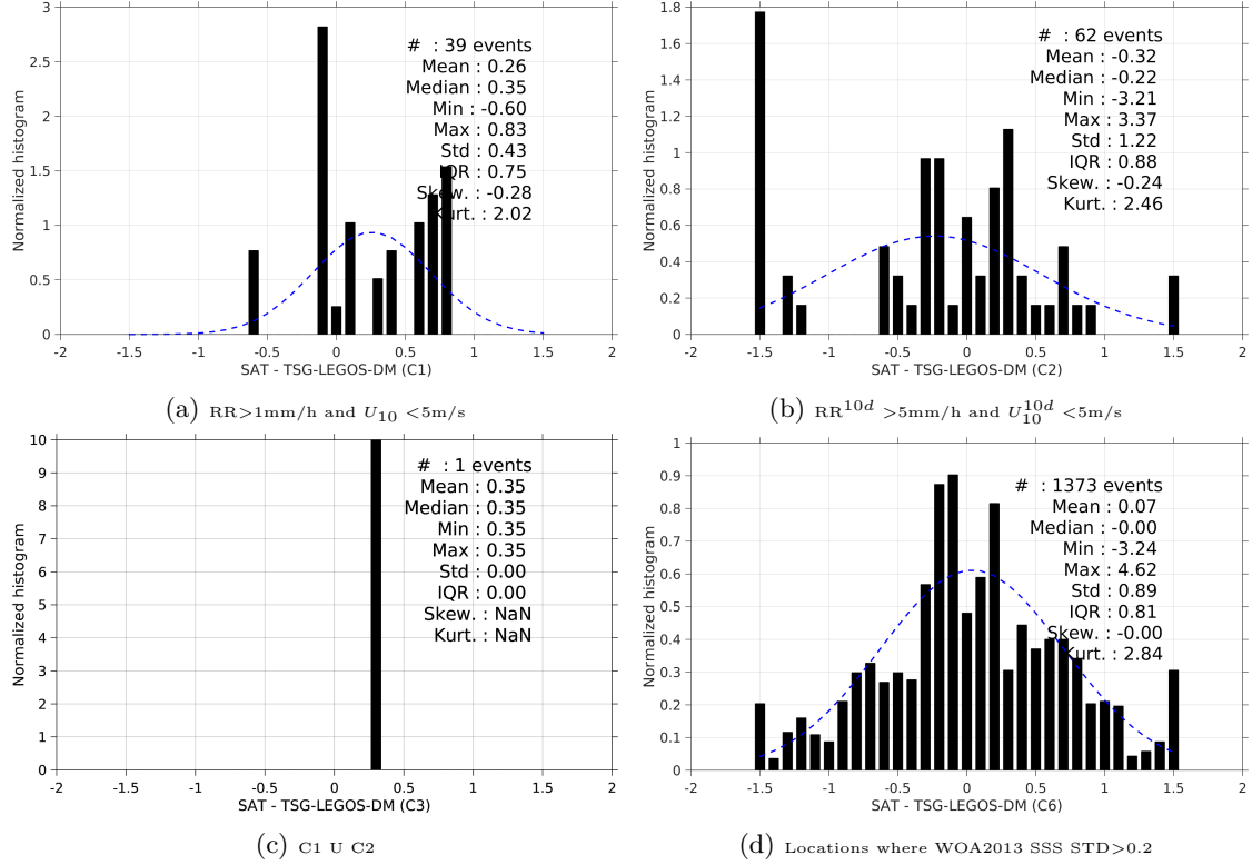
Figure 13: Normalized histogram of \Delta\text{SSS} (SMOS-L3-CATDS-IFREMER-CECOS-V2-MONTHLY-0.25DEG - TSG-LEGOS-DM) for 6 different subdatasets corresponding to: RR > 1\text{mm/h} and U_{10} < 5\text{m/s} (a), RR^{10d} > 5\text{mm/h} and U_{10}^{10d} < 5\text{m/s} (b), C1 U C2 (c), Locations where WOA2013 SSS STD > 0.2 (d).
