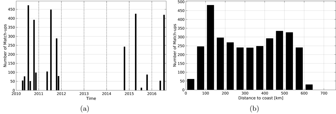
Figure 1: Number of match-ups between TSG-LEGOS-DM and SMOS-L3-CATDS-IFREMER-CECOS-V2-MONTHLY-0.25DEG SSS as a function of time (a) and as function of the distance to coast (b) over the Ganga and Brahmaputra river plumes Pi-MEP region and for the full satellite product period.
