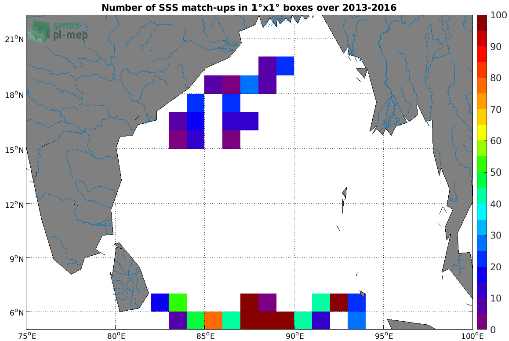
Figure 3: Number of SSS match-ups between Surface drifters SSS and the SMOS SSS L3 v2 - Monthly - 0.25 Deg (CATDS-CECOS-IFREMER) SSS product for the Ganga and Brahmaputra river plumes Pi-MEP region over 1^\circ \times 1^\circ boxes and for the full satellite product period.
