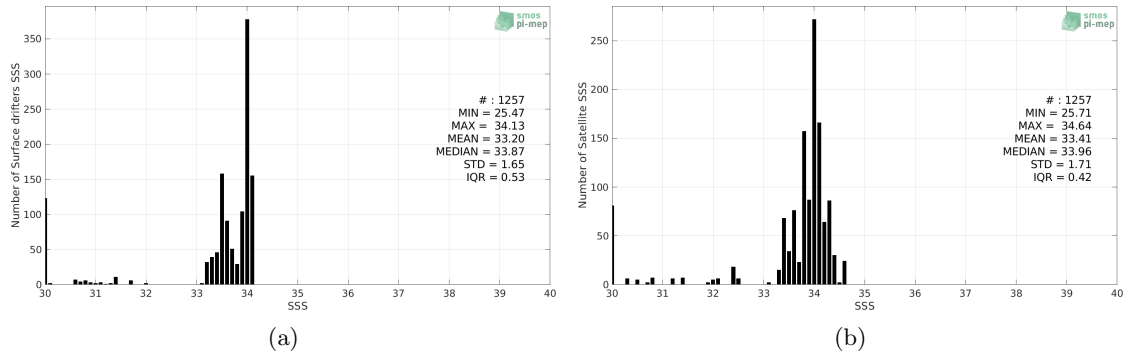
Figure 2: Histograms of SSS from Surface drifters (a) and SMOS SSS L3 v2 - Monthly - 0.25 Deg (CATDS-CECOS-IFREMER) (b) considering all match-up pairs per bins of 0.1 over the Ganga and Brahmaputra river plumes Pi-MEP region and for the full satellite product period.
