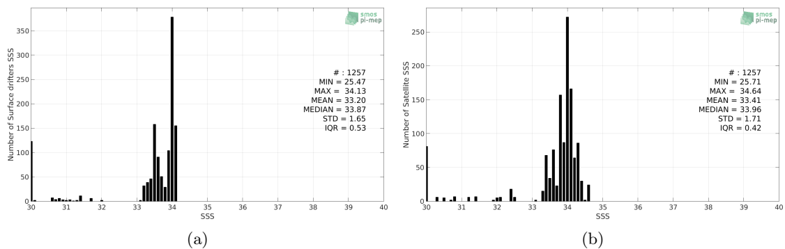
Figure 2: Histograms of SSS from Surface drifters (a) and SMOS-L3-CATDS-IFREMER-CECOS-V2-MONTHLY-0.25DEG (b) considering all match-up pairs per bins of 0.1 over the Ganga and Brahmaputra river plumes Pi-MEP region and for the full satellite product period.
