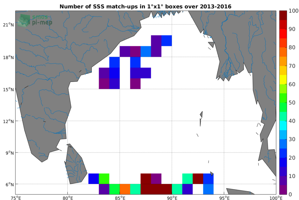
Figure 3: Number of SSS match-ups between Surface drifters SSS and the SMOS-L3-CATDS-IFREMER-CECOS-V2-MONTHLY-0.25DEG SSS product for the Ganga and Brahmaputra river plumes Pi-MEP region over 1°x1° boxes and for the full satellite product period.
