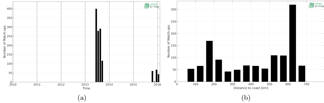
Figure 1: Number of match-ups between Surface drifters and SMOS-L3-CATDS-IFREMER-CECOS-V2-MONTHLY-0.25DEG SSS as a function of time (a) and as function of the distance to coast (b) over the Ganga and Brahmaputra river plumes Pi-MEP region and for the full satellite product period.
