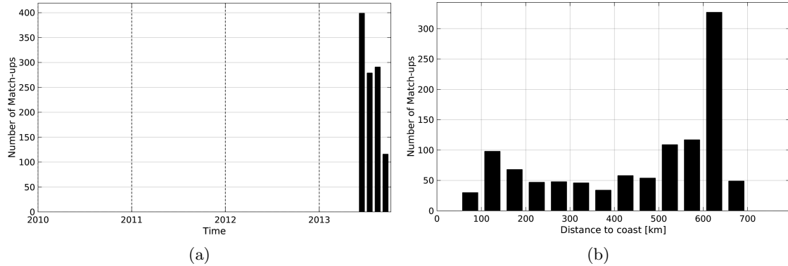
Figure 1: Number of match-ups between Surface drifters and SMOS-L3-CATDS-IFREMER-CECOS-V2-MONTHLY-0.25DEG SSS as a function of time (a) and as function of the distance to coast (b) over the Ganga and Brahmaputra river plumes Pi-MEP region and for the full satellite product period.
