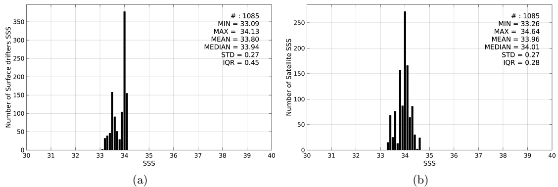
Figure 2: Histograms of SSS from Surface drifters (a) and SMOS-L3-CATDS-IFREMER-CECOS-V2-MONTHLY-0.25DEG (b) considering all match-up pairs per bins of 0.1 over the Ganga and Brahmaputra river plumes Pi-MEP region and for the full satellite product period.
