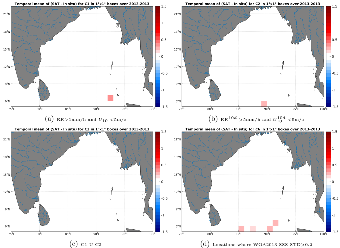
Figure 11: Temporal mean gridded over spatial boxes of size 1°x1° of \Delta SSS (SMOS-L3-CATDS-IFREMER-CECOS-V2-MONTHLY-0.25DEG - Surface drifters) for 4 different subdatasets corresponding to:RR>1mm/h and U_{10} < 5m/s (a), RR^{10d} > 5mm/h and U_{10}^{10d} < 5m/s (b), C1 U C2 (c),Locations where WOA2013 SSS STD>0.2 (d).
