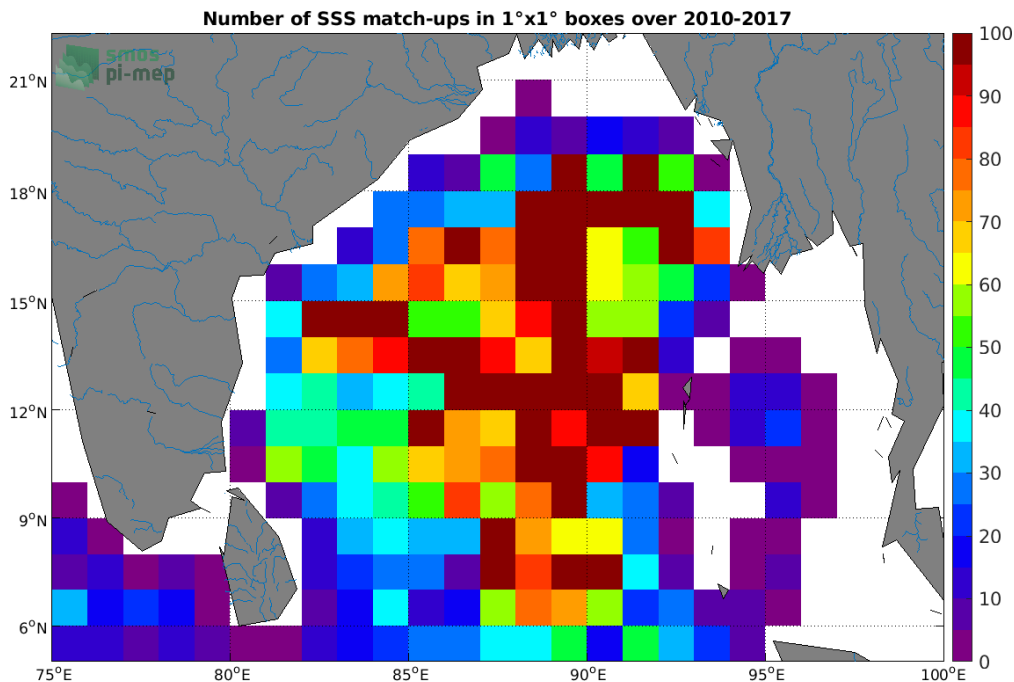
Figure 4: Number of SSS match-ups between Argo SSS and the SMOS SSS L3 v2 - Monthly - 0.25 Deg (CATDS-CECOS-IFREMER) SSS product for the Ganga and Brahmaputra river plumes Pi-MEP region over 1^\circ \times 1^\circ boxes and for the full satellite product period.
