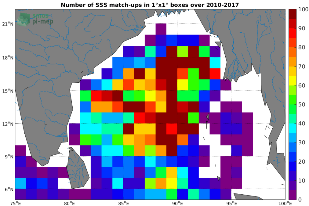
Figure 4: Number of SSS match-ups between Argo SSS and the SMOS-L3-CATDS-IFREMER-CECOS-V2-MONTHLY-0.25DEG SSS product for the Ganga and Brahmaputra river plumes Pi-MEP region over 1°x1° boxes and for the full satellite product period.
