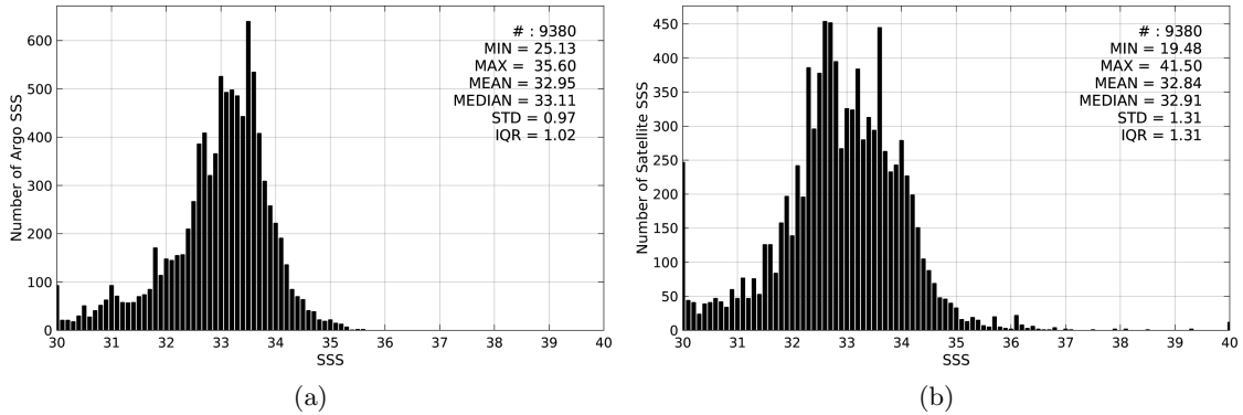
Figure 2: Histograms of SSS from Argo (a) and SMOS-L3-CATDS-IFREMER-CECOS-V2-MONTHLY-0.25DEG (b) considering all match-up pairs per bins of 0.1 over the Ganga and Brahmaputra river plumes Pi-MEP region and for the full satellite product period.
