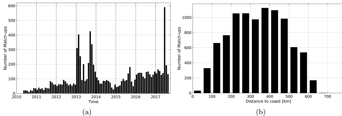
Figure 1: Number of match-ups between Argo and SMOS-L3-CATDS-IFREMER-CECOS-V2-MONTHLY-0.25DEG SSS as a function of time (a) and as function of the distance to coast (b) over the Ganga and Brahmaputra river plumes Pi-MEP region and for the full satellite product period.
