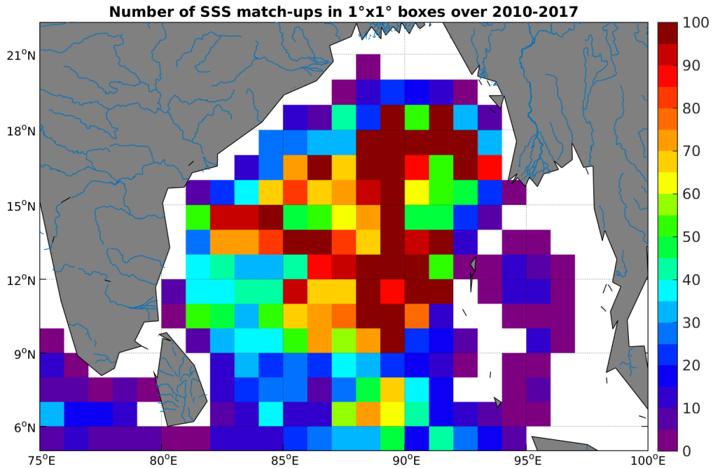
Figure 4: Number of SSS match-ups between Argo SSS and the SMOS-L3-CATDS-IFREMER-CECOS-V2-MONTHLY-0.25DEG SSS product for the Ganga and Brahmaputra river plumes Pi-MEP region over 1^\circ \times 1^\circ boxes and for the full satellite product period.
