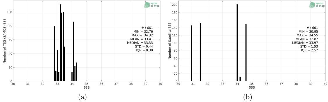
Figure 2: Histograms of SSS from TSG (SAMOS) (a) and SMOS SSS L3 v2 - Daily - 0.5 Deg (CATDS-CECOS-IFREMER) (b) considering all match-up pairs per bins of 0.1 over the Ganga and Brahmaputra river plumes Pi-MEP region and for the full satellite product period.
