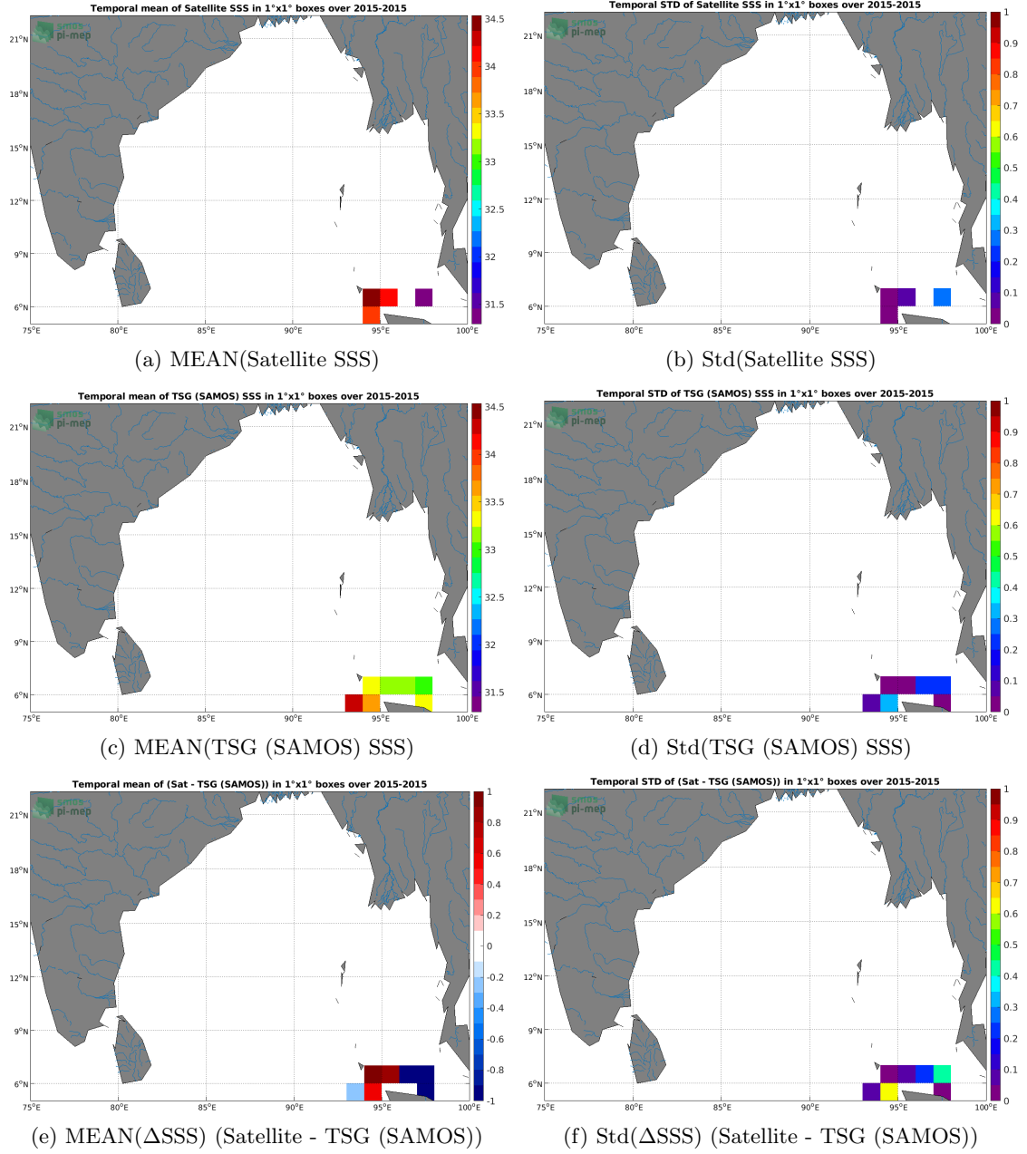
Figure 6: Temporal mean (left) and Std (right) of SSS from SMOS SSS L3 v2 - Daily - 0.5 Deg (CATDS-CECOS-IFREMER) (top), TSG (SAMOS) (middle), and of \Delta SSS (Satellite - TSG (SAMOS)). Only match-up pairs are used to generate these maps.
