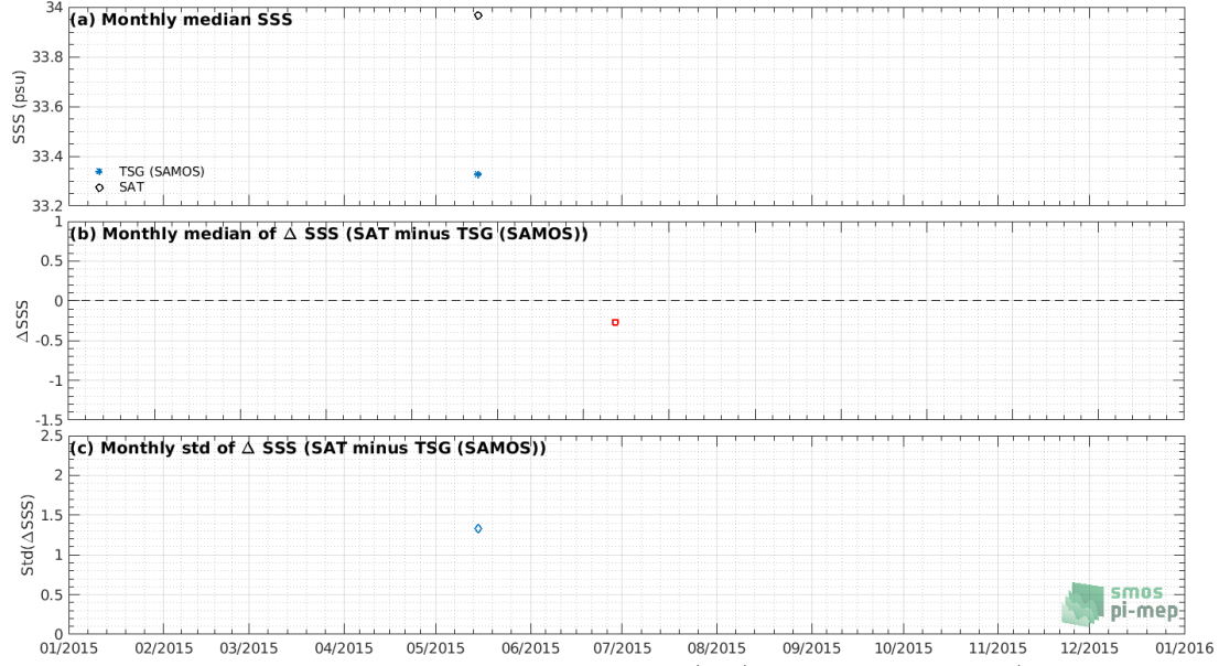
Figure 7: Time series of the monthly median SSS (top), median of \Delta SSS (Satellite - TSG (SAMOS)) and Std of \Delta SSS (Satellite - TSG (SAMOS)) over the Ganga and Brahmaputra river plumes Pi-MEP region considering all match-ups collected by the Pi-MEP.
