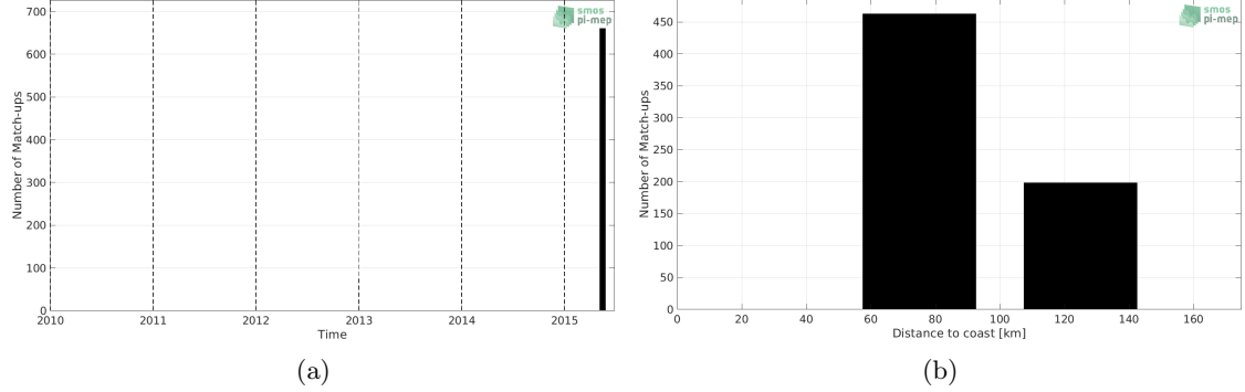
Figure 1: Number of match-ups between TSG (SAMOS) and SMOS SSS L3 v2 - Daily - 0.5 Deg (CATDS-CECOS-IFREMER) SSS as a function of time (a) and as function of the distance to coast (b) over the Ganga and Brahmaputra river plumes Pi-MEP region and for the full satellite product period.
