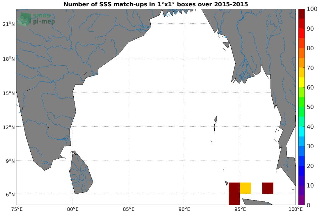
Figure 4: Number of SSS match-ups between TSG (SAMOS) SSS and the SMOS SSS L3 v2 - Daily - 0.5 Deg (CATDS-CECOS-IFREMER) SSS product for the Ganga and Brahmaputra river plumes Pi-MEP region over 1^\circ \times 1^\circ boxes and for the full satellite product period.
