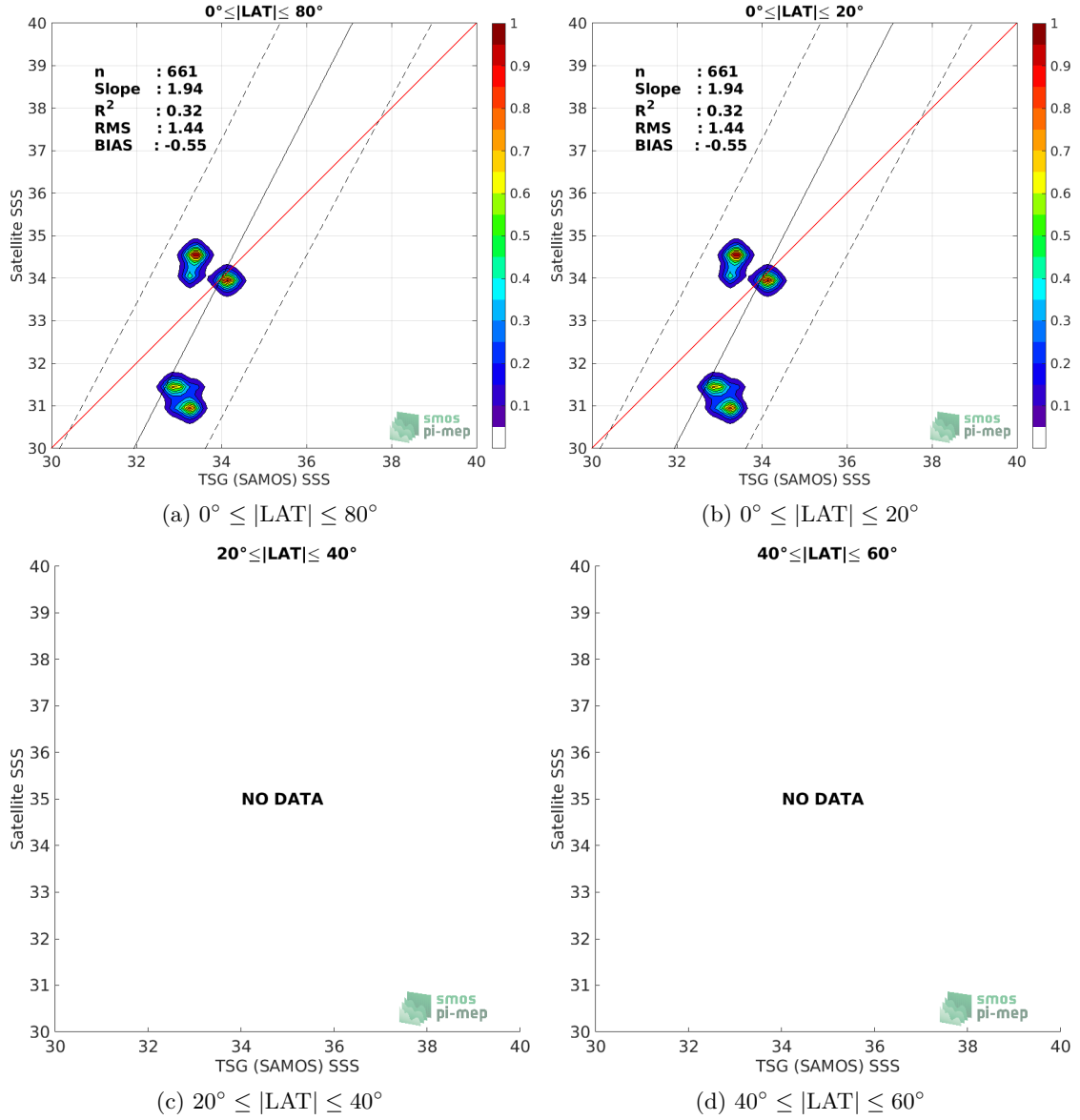
Figure 9: Contour maps of the concentration of SMOS SSS L3 v2 - Daily - 0.5 Deg (CATDS-CECOS-IFREMER) SSS (y-axis) versus TSG (SAMOS) SSS (x-axis) at match-up pairs for different latitude bands. For each plot, the red line shows x=y . The black thin and dashed lines indicate a linear fit through the data cloud and the \pm 95\% confidence levels, respectively. The number match-up pairs n , the slope and R^2 coefficient of the linear fit, the root mean square (RMS) and the mean bias between satellite and in situ data are indicated for each latitude band in each plots.
