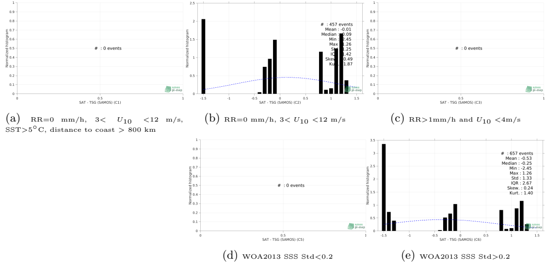
Figure 13: Normalized histogram of \Delta\text{SSS} (SMOS SSS L3 v2 - Daily - 0.5 Deg (CATDS-CECOS-IFREMER) - TSG (SAMOS)) for 5 different subdatasets corresponding to: RR=0 mm/h, 3 < U_{10} < 12 m/s, SST > 5^\circ\text{C} , distance to coast > 800 km (a), RR=0 mm/h, 3 < U_{10} < 12 m/s (b), RR > 1\text{mm/h} and U_{10} < 4\text{m/s} (c), WOA2013 SSS Std < 0.2 (d), WOA2013 SSS Std > 0.2 (e).
