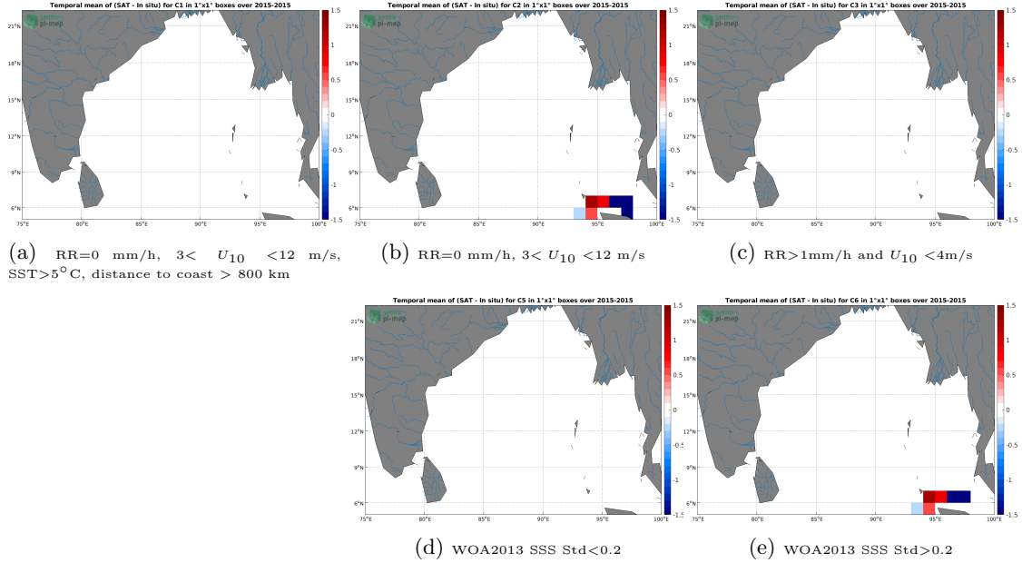
Figure 12: Temporal mean gridded over spatial boxes of size 1^{\circ}\times 1^{\circ} of \Delta\text{SSS} (SMOS SSS L3 v2 - Daily - 0.5 Deg (CATDS-CECOS-IFREMER) - TSG (SAMOS)) for 5 different subdatasets corresponding to: \text{RR}=0 mm/h, 3 < U_{10} < 12 m/s, \text{SST} > 5^{\circ}\text{C} , distance to coast > 800 km (a), \text{RR}=0 mm/h, 3 < U_{10} < 12 m/s (b), \text{RR} > 1 mm/h and U_{10} < 4 m/s (c), WOA2013 SSS Std < 0.2 (d), WOA2013 SSS Std > 0.2 (e).
