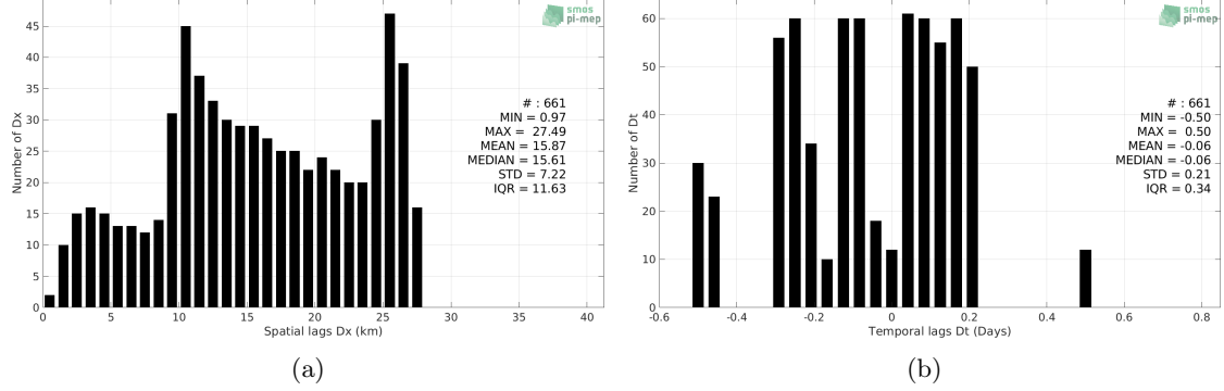
Figure 5: Histograms of the spatial (a) and temporal (b) lags between the location/time of the TSG (SAMOS) measurement and the date of the corresponding SMOS SSS L3 v2 - Daily - 0.5 Deg (CATDS-CECOS-IFREMER) SSS pixel.
