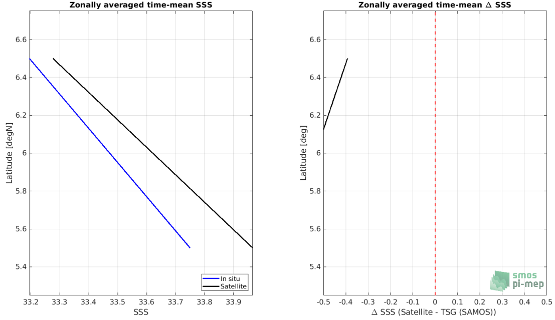
Figure 8: Left panel: Zonal mean SSS from SMOS SSS L3 v2 - Daily - 0.5 Deg (CATDS-CECOS-IFREMER) satellite product (black) and from TSG (SAMOS) (blue). Right panel: Zonal mean of \Delta SSS (Satellite - TSG (SAMOS)) for all the collected Pi-MEP match-up pairs estimated over the full satellite product period.
