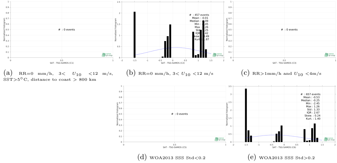
Figure 13: Normalized histogram of \Delta\text{SSS} (SMOS-L3-CATDS-CECOS-IFREMER-V2-1DAY-0.5DEG - TSG-SAMOS) for 5 different subdatasets corresponding to: RR=0 mm/h, 3 < U_{10} < 12 m/s, SST > 5^{\circ}\text{C} , distance to coast > 800 km (a), RR=0 mm/h, 3 < U_{10} < 12 m/s (b), RR > 1\text{mm/h} and U_{10} < 4\text{m/s} (c), WOA2013 SSS Std < 0.2 (d), WOA2013 SSS Std > 0.2 (e).
