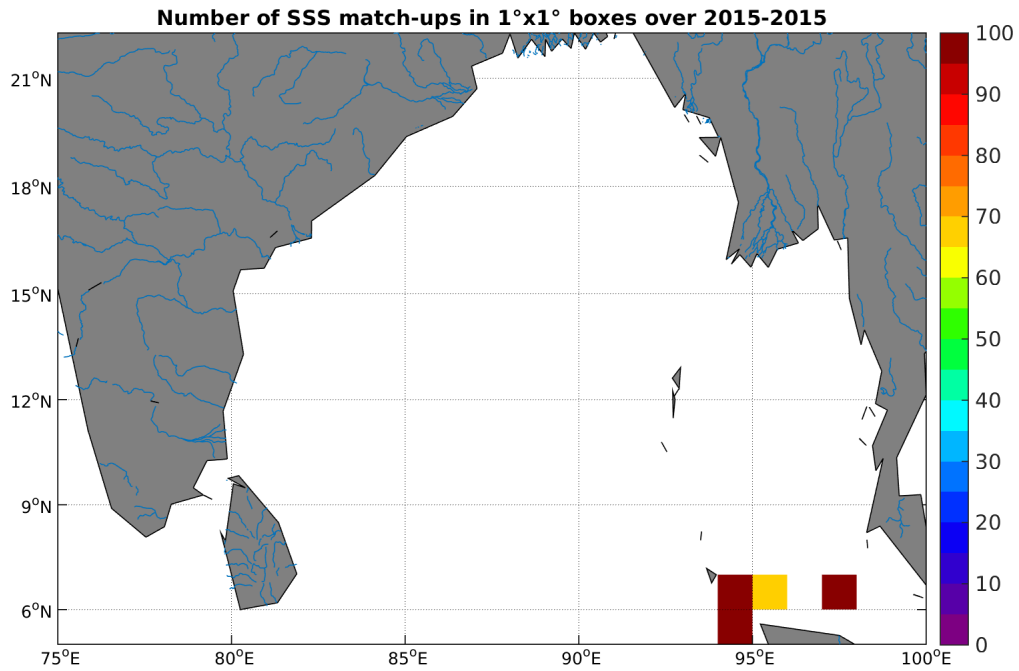
Figure 4: Number of SSS match-ups between TSG-SAMOS SSS and the SMOS-L3-CATDS-CECOS-IFREMER-V2-1DAY-0.5DEG SSS product for the Ganga and Brahmaputra river plumes Pi-MEP region over 1^\circ \times 1^\circ boxes and for the full satellite product period.
