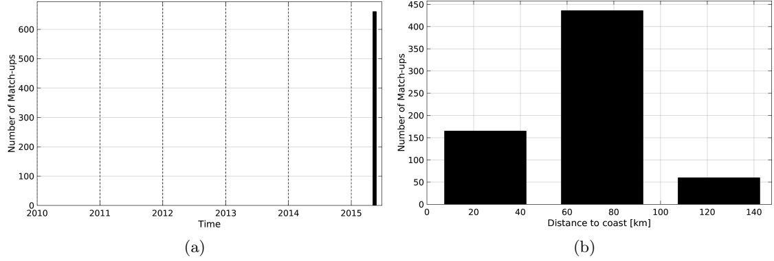
Figure 1: Number of match-ups between TSG-SAMOS and SMOS-L3-CATDS-CECOS-IFREMER-V2-1DAY-0.5DEG SSS as a function of time (a) and as function of the distance to coast (b) over the Ganga and Brahmaputra river plumes Pi-MEP region and for the full satellite product period.
