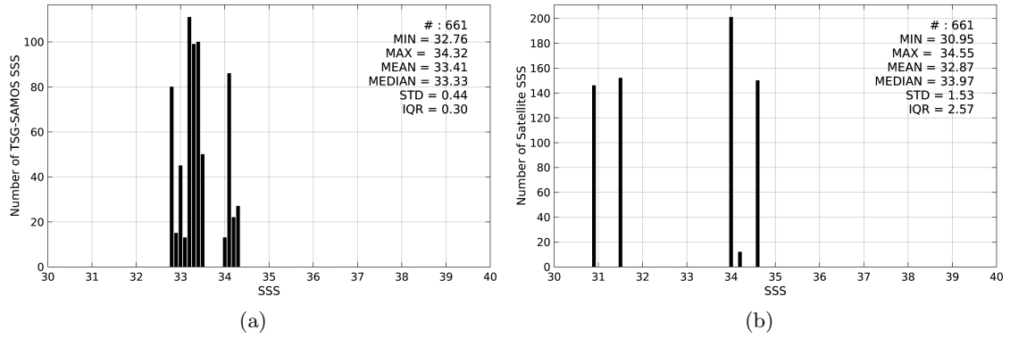
Figure 2: Histograms of SSS from TSG-SAMOS (a) and SMOS-L3-CATDS-CECOS-IFREMER-V2-1DAY-0.5DEG (b) considering all match-up pairs per bins of 0.1 over the Ganga and Brahmaputra river plumes Pi-MEP region and for the full satellite product period.
