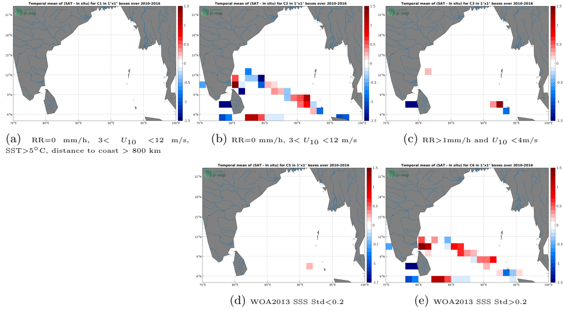
Figure 12: Temporal mean gridded over spatial boxes of size 1^\circ \times 1^\circ of \Delta SSS (SMOS-L3-CATDS-CECOS-IFREMER-V2-1DAY-0.5DEG - TSG-LEGOS-DM) for 5 different subdatasets corresponding to: RR=0 mm/h, 3 < U_{10} < 12 m/s, SST > 5^\circ C , distance to coast > 800 km (a), RR=0 mm/h, 3 < U_{10} < 12 m/s (b), RR > 1 mm/h and U_{10} < 4 m/s (c), WOA2013 SSS Std < 0.2 (d), WOA2013 SSS Std > 0.2 (e).
