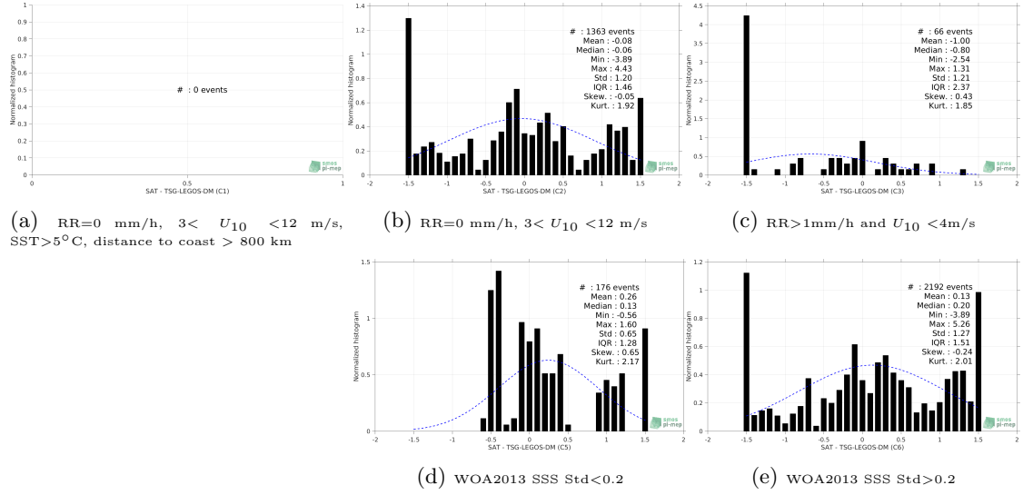
Figure 13: Normalized histogram of \Delta\text{SSS} (SMOS-L3-CATDS-CECOS-IFREMER-V2-1DAY-0.5DEG - TSG-LEGOS-DM) for 5 different subdatasets corresponding to: RR=0 mm/h, 3 < U_{10} < 12 m/s, SST > 5^\circ\text{C} , distance to coast > 800 km (a), RR=0 mm/h, 3 < U_{10} < 12 m/s (b), RR > 1\text{mm/h} and U_{10} < 4\text{m/s} (c), WOA2013 SSS Std <0.2 (d), WOA2013 SSS Std >0.2 (e).
