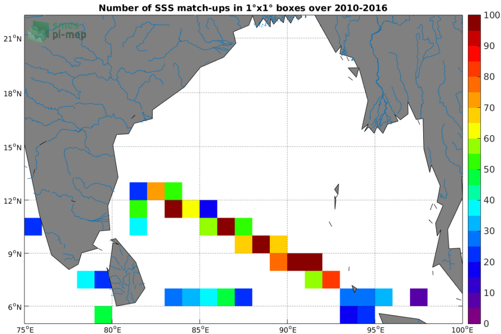
Figure 4: Number of SSS match-ups between TSG-LEGOS-DM SSS and the SMOS-L3-CATDS-CECOS-IFREMER-V2-1DAY-0.5DEG SSS product for the Ganga and Brahmaputra river plumes Pi-MEP region over 1^{\circ} \times 1^{\circ} boxes and for the full satellite product period.
