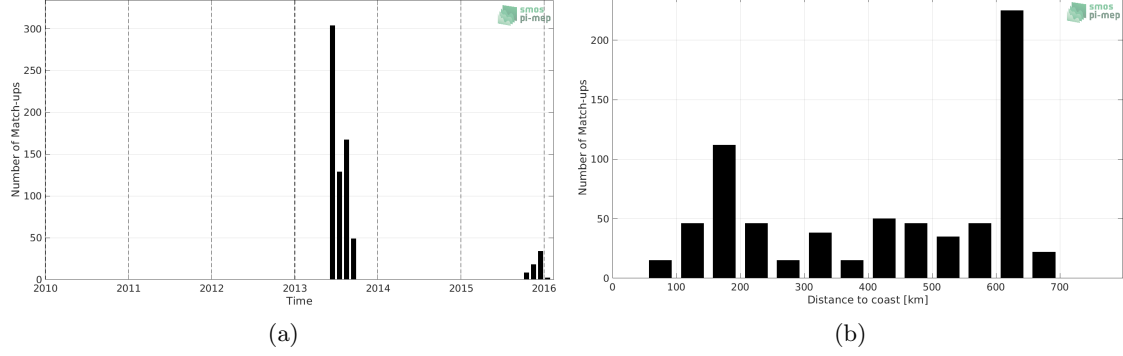
Figure 1: Number of match-ups between Surface drifters and SMOS SSS L3 v2 - Daily - 0.5 Deg (CATDS-CECOS-IFREMER) SSS as a function of time (a) and as function of the distance to coast (b) over the Ganga and Brahmaputra river plumes Pi-MEP region and for the full satellite product period.
