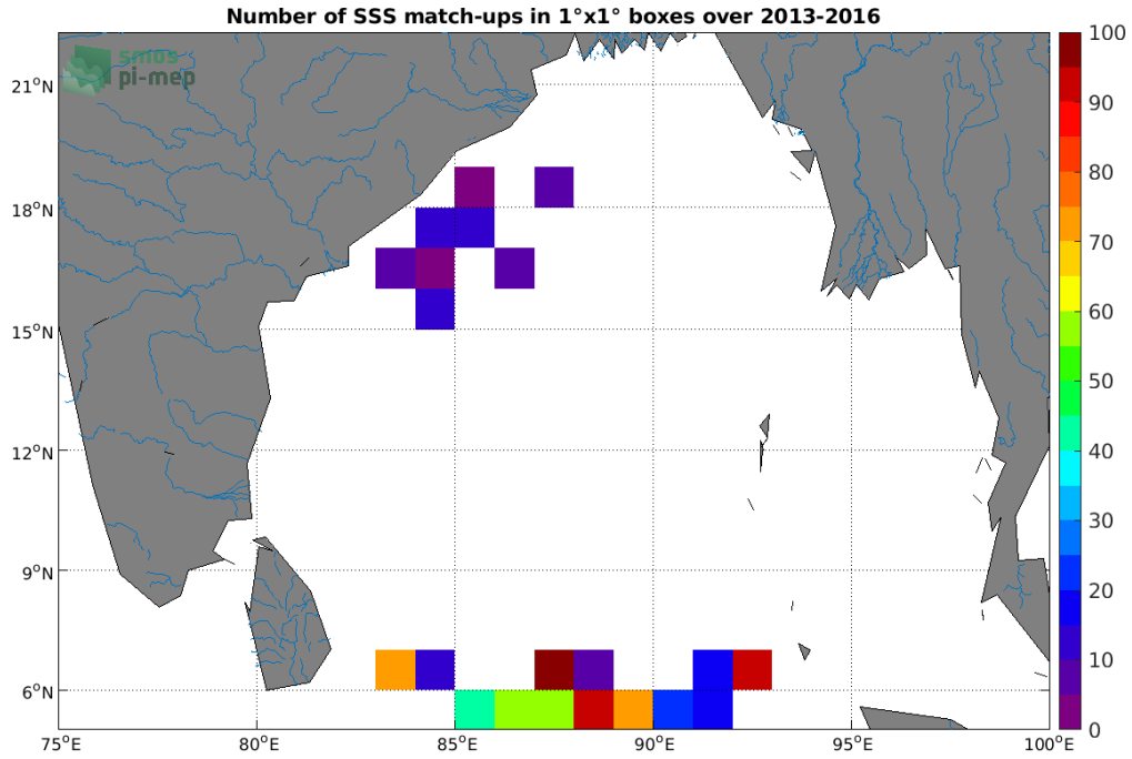
Figure 3: Number of SSS match-ups between Surface drifters SSS and the SMOS SSS L3 v2 - Daily - 0.5 Deg (CATDS-CECOS-IFREMER) SSS product for the Ganga and Brahmaputra river plumes Pi-MEP region over 1°x1° boxes and for the full satellite product period.
