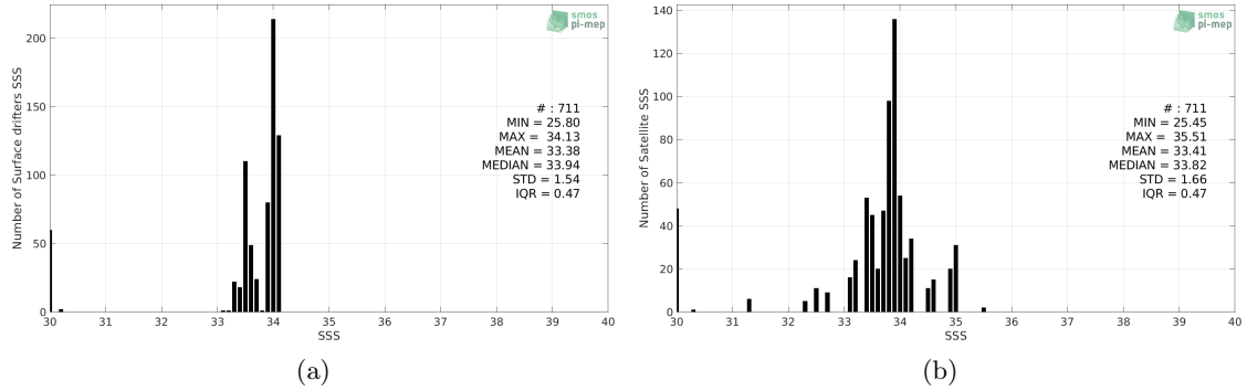
Figure 2: Histograms of SSS from Surface drifters (a) and SMOS SSS L3 v2 - Daily - 0.5 Deg (CATDS-CECOS-IFREMER) (b) considering all match-up pairs per bins of 0.1 over the Ganga and Brahmaputra river plumes Pi-MEP region and for the full satellite product period.
