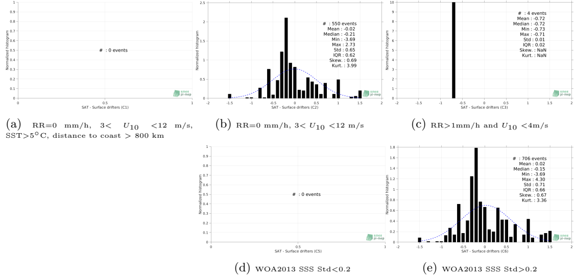
Figure 12: Normalized histogram of \Delta\text{SSS} (SMOS L3 v2 - Daily - 0.5 Deg (CATDS-CECOS-IFREMER) - Surface drifters) for 5 different subdatasets corresponding to: RR=0 mm/h, 3 < U_{10} < 12 m/s, SST > 5^\circ\text{C} , distance to coast > 800 km (a), RR=0 mm/h, 3 < U_{10} < 12 m/s (b), RR > 1\text{mm/h} and U_{10} < 4\text{m/s} (c), WOA2013 SSS Std <0.2 (d), WOA2013 SSS Std >0.2 (e).
