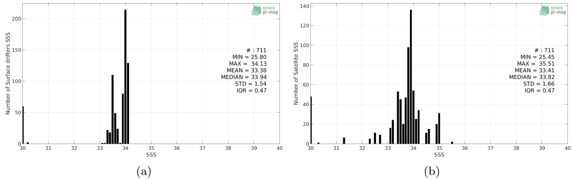
Figure 2: Histograms of SSS from Surface drifters (a) and SMOS L3 v2 - Daily - 0.5 Deg (CATDS-CECOS-IFREMER) (b) considering all match-up pairs per bins of 0.1 over the Ganga and Brahmaputra river plumes Pi-MEP region and for the full satellite product period.
