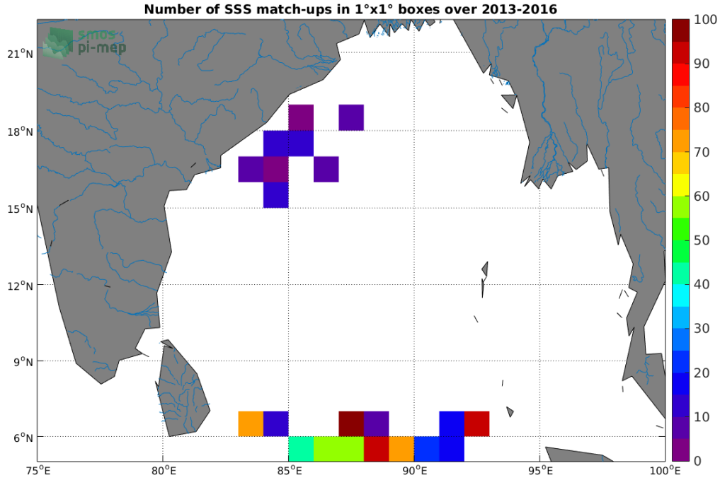
Figure 3: Number of SSS match-ups between Surface drifters SSS and the SMOS L3 v2 - Daily - 0.5 Deg (CATDS-CECOS-IFREMER) SSS product for the Ganga and Brahmaputra river plumes Pi-MEP region over 1^\circ \times 1^\circ boxes and for the full satellite product period.
