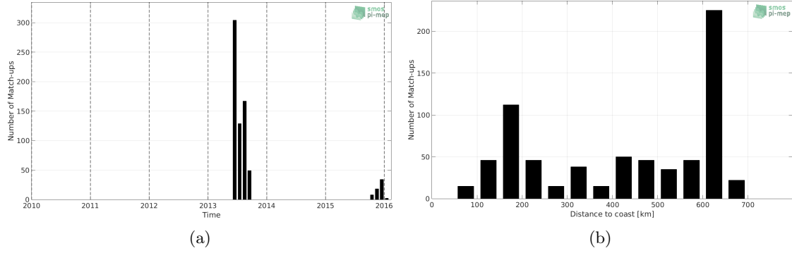
Figure 1: Number of match-ups between Surface drifters and SMOS L3 v2 - Daily - 0.5 Deg (CATDS-CECOS-IFREMER) SSS as a function of time (a) and as function of the distance to coast (b) over the Ganga and Brahmaputra river plumes Pi-MEP region and for the full satellite product period.
