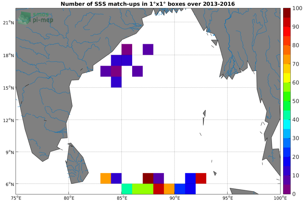
Figure 3: Number of SSS match-ups between Surface drifters SSS and the SMOS-L3-CATDS-CECOS-IFREMER-V2-1DAY-0.5DEG SSS product for the Ganga and Brahmaputra river plumes Pi-MEP region over 1^\circ \times 1^\circ boxes and for the full satellite product period.
