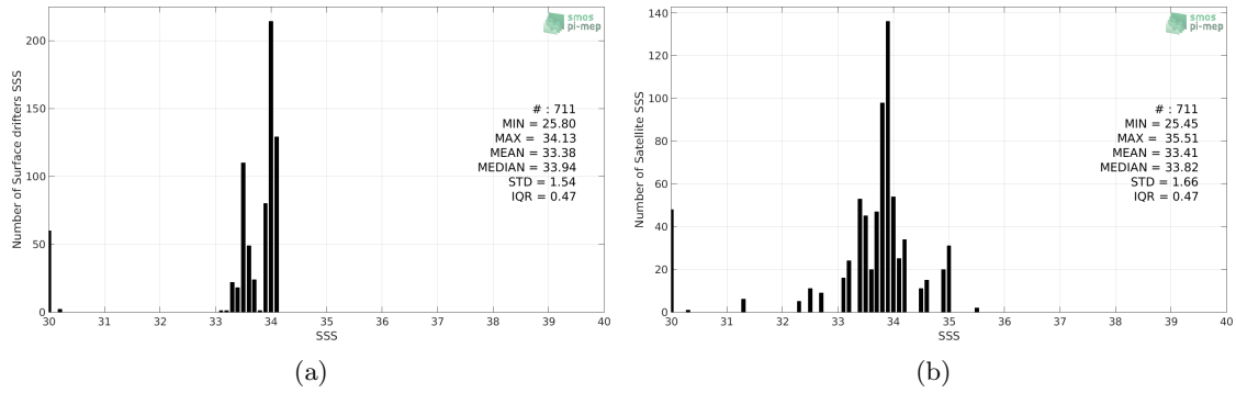
Figure 2: Histograms of SSS from Surface drifters (a) and SMOS-L3-CATDS-CECOS-IFREMER-V2-1DAY-0.5DEG (b) considering all match-up pairs per bins of 0.1 over the Ganga and Brahmaputra river plumes Pi-MEP region and for the full satellite product period.
