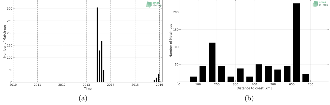
Figure 1: Number of match-ups between Surface drifters and SMOS-L3-CATDS-CECOS-IFREMER-V2-1DAY-0.5DEG SSS as a function of time (a) and as function of the distance to coast (b) over the Ganga and Brahmaputra river plumes Pi-MEP region and for the full satellite product period.
