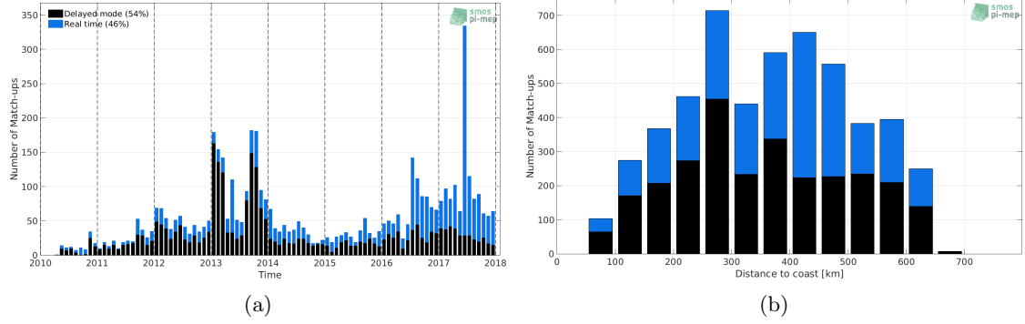
Figure 1: Number of match-ups between Argo and SMOS SSS L3 v2 - Daily - 0.5 Deg (CATDS-CECOS-IFREMER) SSS as a function of time (a) and as function of the distance to coast (b) over the Ganga and Brahmaputra river plumes Pi-MEP region and for the full satellite product period.
