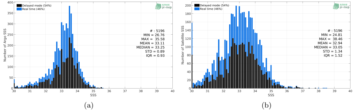
Figure 2: Histograms of SSS from Argo (a) and SMOS SSS L3 v2 - Daily - 0.5 Deg (CATDS-CECOS-IFREMER) (b) considering all match-up pairs per bins of 0.1 over the Ganga and Brahmaputra river plumes Pi-MEP region and for the full satellite product period.
