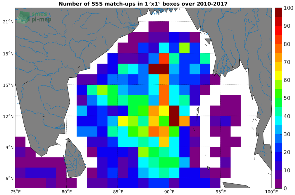
Figure 4: Number of SSS match-ups between Argo SSS and the SMOS SSS L3 v2 - Daily - 0.5 Deg (CATDS-CECOS-IFREMER) SSS product for the Ganga and Brahmaputra river plumes Pi-MEP region over 1°x1° boxes and for the full satellite product period.
