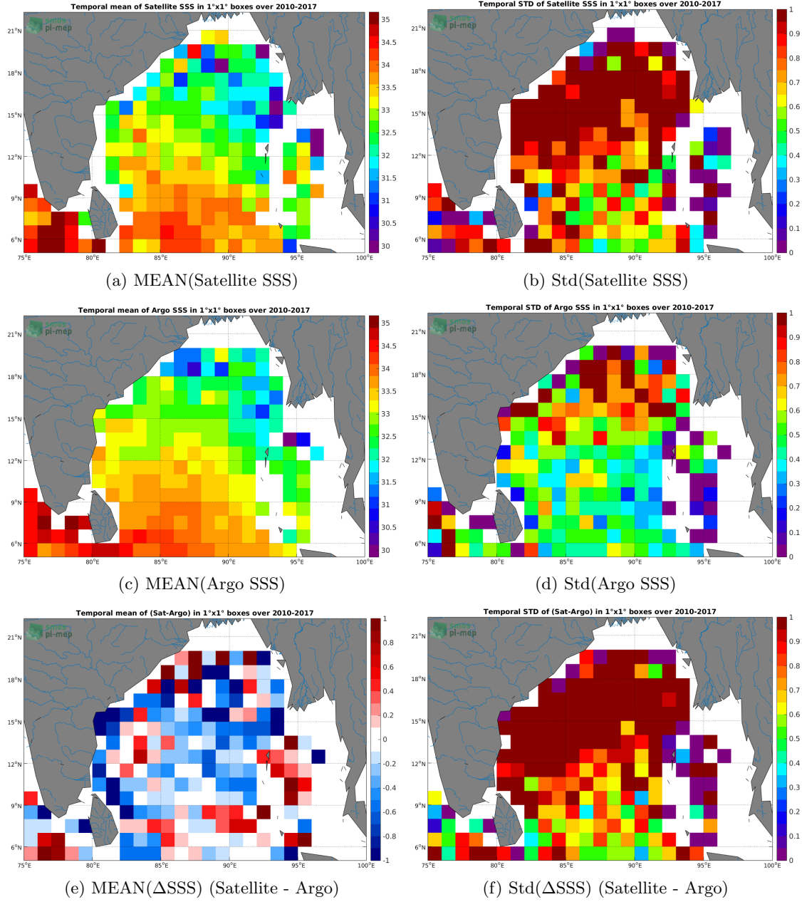
Figure 6: Temporal mean (left) and Std (right) of SSS from SMOS-L3-CATDS-CECOS-IFREMER-V2-1DAY-0.5DEG (top), Argo (middle), and of ΔSSS (Satellite - Argo). Only match-up pairs are used to generate these maps.
