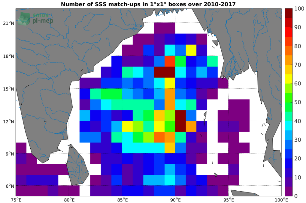
Figure 4: Number of SSS match-ups between Argo SSS and the SMOS-L3-CATDS-CECOS-IFREMER-V2-1DAY-0.5DEG SSS product for the Ganga and Brahmaputra river plumes Pi-MEP region over 1°x1° boxes and for the full satellite product period.
