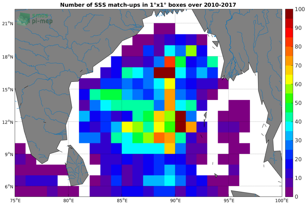
Figure 4: Number of SSS match-ups between Argo SSS and the SMOS-L3-CATDS-CECOS-IFREMER-V2-1DAY-0.5DEG SSS product for the Ganga and Brahmaputra river plumes Pi-MEP region over 1^{\circ} \times 1^{\circ} boxes and for the full satellite product period.
