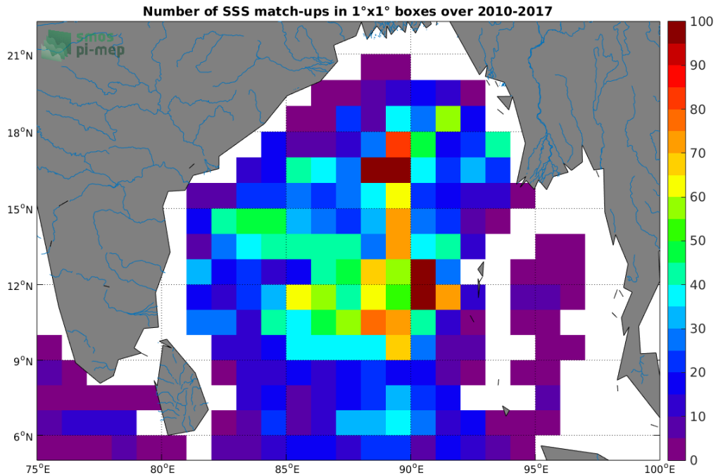
Figure 4: Number of SSS match-ups between Argo SSS and the SMOS-L3-CATDS-CECOS-IFREMER-V2-1DAY-0.5DEG SSS product for the Ganga and Brahmaputra river plumes Pi-MEP region over 1^\circ \times 1^\circ boxes and for the full satellite product period.
