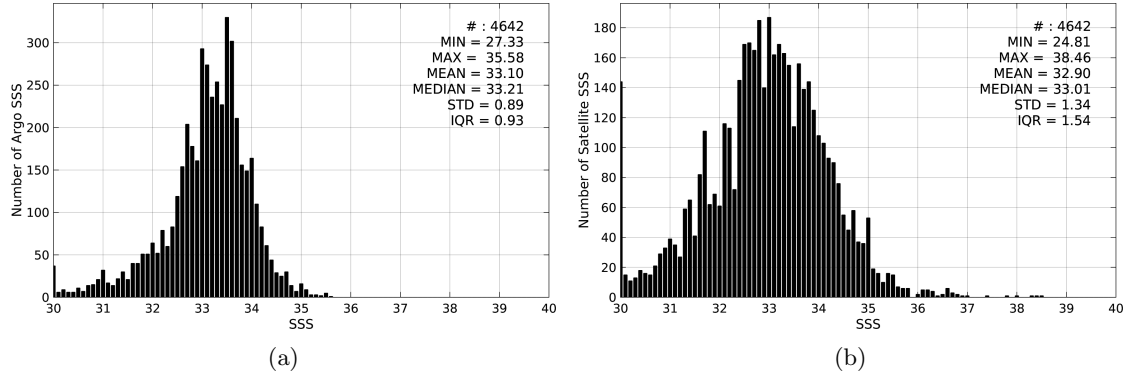
Figure 2: Histograms of SSS from Argo (a) and SMOS-L3-CATDS-CECOS-IFREMER-V2-1DAY-0.5deg (b) considering all match-up pairs per bins of 0.1 over the Ganga and Brahmaputra river plumes Pi-MEP region and for the full satellite product period.
