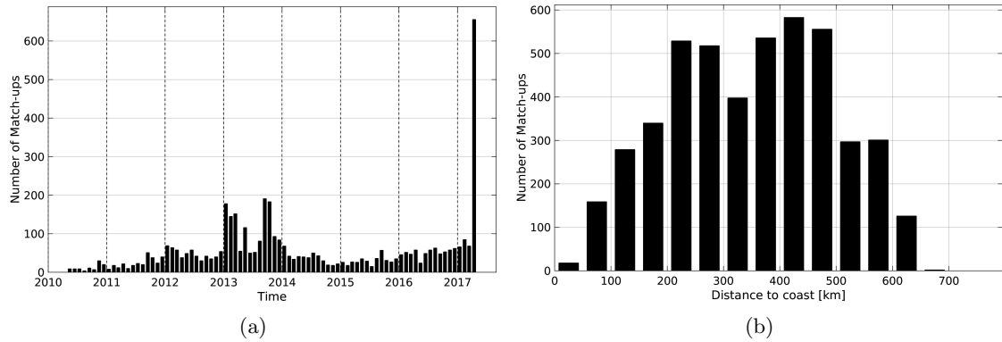
Figure 1: Number of match-ups between Argo and SMOS-L3-CATDS-CECOS-IFREMER-V2-1DAY-0.5deg SSS as a function of time (a) and as function of the distance to coast (b) over the Ganga and Brahmaputra river plumes Pi-MEP region and for the full satellite product period.
