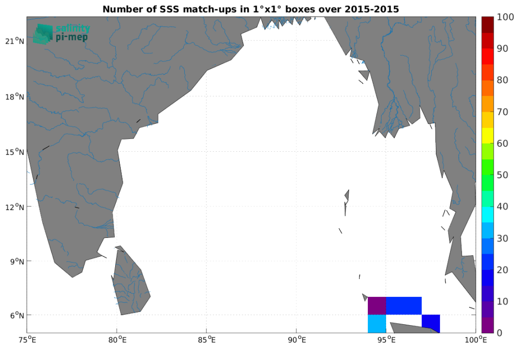
Figure 5: Number of SSS match-ups between TSG (SAMOS) SSS and the SMOS SSS L3 v335 - Monthly - 25 km (CATDS-CPDC) SSS product for the Ganga and Brahmaputra river plumes Pi-MEP region over 1°x1° boxes and for the full satellite product period.
