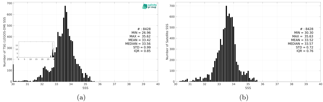
Figure 3: Histograms of SSS from TSG (LEGOS-DM) (a) and SMOS SSS L3 v335 - Monthly - 25 km (CATDS-CPDC) (b) considering all match-up pairs per bins of 0.1 over the Ganga and Brahmaputra river plumes Pi-MEP region and for the full satellite product period.
