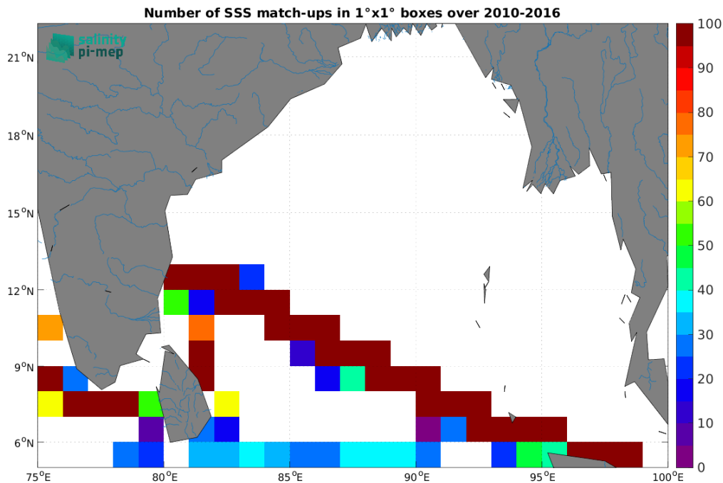
Figure 5: Number of SSS match-ups between TSG (LEGOS-DM) SSS and the SMOS SSS L3 v335 - Monthly - 25 km (CATDS-CPDC) SSS product for the Ganga and Brahmaputra river plumes Pi-MEP region over 1^\circ \times 1^\circ boxes and for the full satellite product period.
