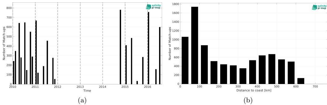
Figure 2: Number of match-ups between TSG (LEGOS-DM) and SMOS SSS L3 v335 - Monthly - 25 km (CATDS-CPDC) SSS as a function of time (a) and as function of the distance to coast (b) over the Ganga and Brahmaputra river plumes Pi-MEP region and for the full satellite product period.
