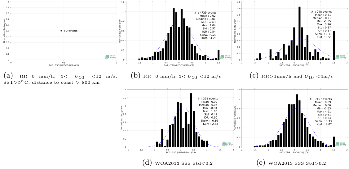
Figure 13: Normalized histogram of \Delta SSS (SMOS SSS L3 v335 - Monthly - 25 km (CATDS-CPDC) - TSG (LEGOS-DM)) for 5 different subdatasets corresponding to: RR=0 mm/h, 3 < U_{10} < 12 m/s, SST > 5^\circ\text{C} , distance to coast > 800 km (a), RR=0 mm/h, 3 < U_{10} < 12 m/s (b), RR > 1 mm/h and U_{10} < 4 m/s (c), WOA2013 SSS Std < 0.2 (d), WOA2013 SSS Std > 0.2 (e).
