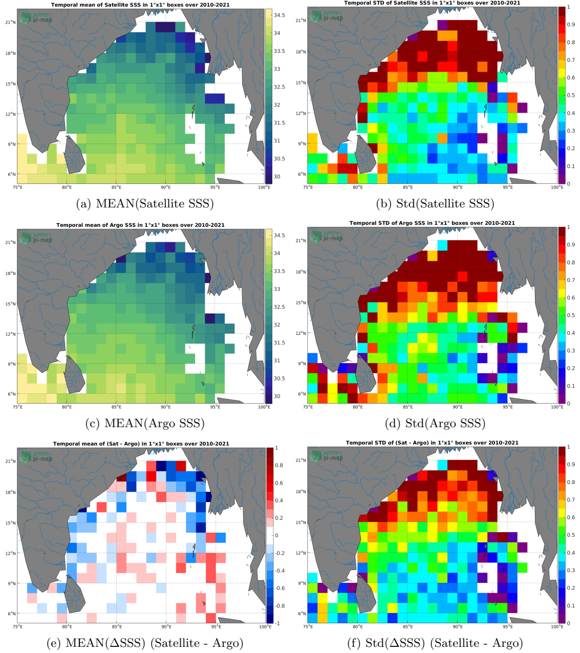
Figure 6: Temporal mean (left) and Std (right) of SSS from SMOS SSS L3 v335 - Monthly - 25 km (CATDS-CPDC) (top), Argo (middle), and of ΔSSS (Satellite - Argo). Only match-up pairs are used to generate these maps.
