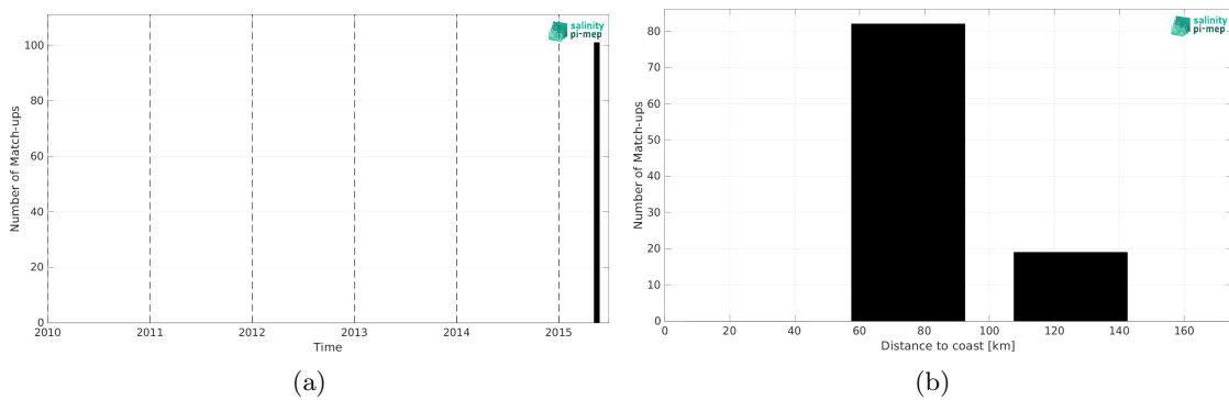
Figure 2: Number of match-ups between TSG (SAMOS) and SMOS SSS L3 v335 - 10 Days - 25 km (CATDS-CPDC) SSS as a function of time (a) and as function of the distance to coast (b) over the Ganga and Brahmaputra river plumes Pi-MEP region and for the full satellite product period.
