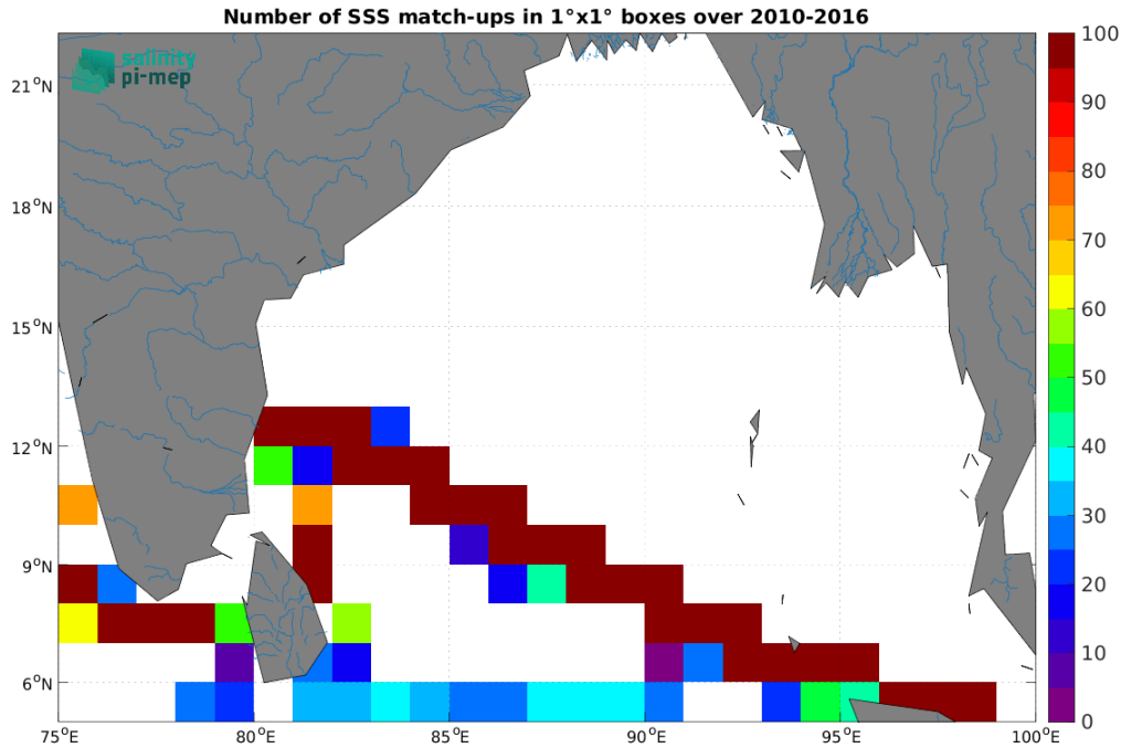
Figure 5: Number of SSS match-ups between TSG (LEGOS-DM) SSS and the SMOS SSS L3 v335 - 10 Days - 25 km (CATDS-CPDC) SSS product for the Ganga and Brahmaputra river plumes Pi-MEP region over 1^{\circ} \times 1^{\circ} boxes and for the full satellite product period.
