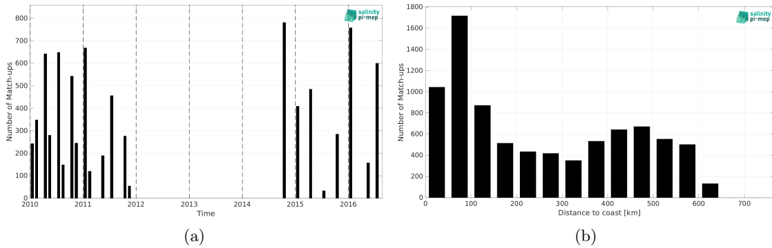
Figure 2: Number of match-ups between TSG (LEGOS-DM) and SMOS SSS L3 v335 - 10 Days - 25 km (CATDS-CPDC) SSS as a function of time (a) and as function of the distance to coast (b) over the Ganga and Brahmaputra river plumes Pi-MEP region and for the full satellite product period.
