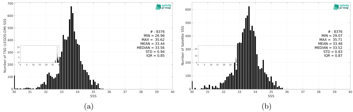
Figure 3: Histograms of SSS from TSG (LEGOS-DM) (a) and SMOS SSS L3 v335 - 10 Days - 25 km (CATDS-CPDC) (b) considering all match-up pairs per bins of 0.1 over the Ganga and Brahmaputra river plumes Pi-MEP region and for the full satellite product period.
