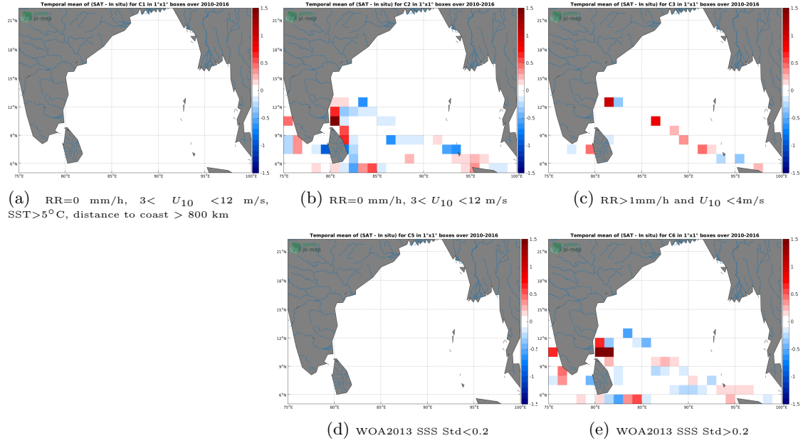
Figure 12: Temporal mean gridded over spatial boxes of size 1^{\circ} \times 1^{\circ} of \Delta\text{SSS} (SMOS SSS L3 v335 - 10 Days - 25 km (CATDS-CPDC) - TSG (LEGOS-DM)) for 5 different subdatasets corresponding to: RR=0 mm/h, 3 < U_{10} < 12 m/s, SST >5^{\circ}\text{C} , distance to coast > 800 km (a), RR=0 mm/h, 3 < U_{10} < 12 m/s (b), RR >1 mm/h and U_{10} < 4 m/s (c), WOA2013 SSS Std <0.2 (d), WOA2013 SSS Std >0.2 (e).
