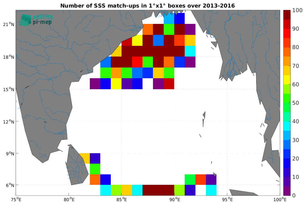
Figure 4: Number of SSS match-ups between Surface drifters SSS and the SMOS SSS L3 v335 - 10 Days - 25 km (CATDS-CPDC) SSS product for the Ganga and Brahmaputra river plumes Pi-MEP region over 1^\circ \times 1^\circ boxes and for the full satellite product period.
