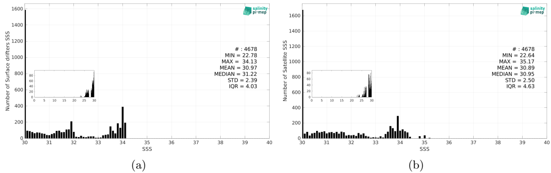
Figure 3: Histograms of SSS from Surface drifters (a) and SMOS SSS L3 v335 - 10 Days - 25 km (CATDS-CPDC) (b) considering all match-up pairs per bins of 0.1 over the Ganga and Brahmaputra river plumes Pi-MEP region and for the full satellite product period.
