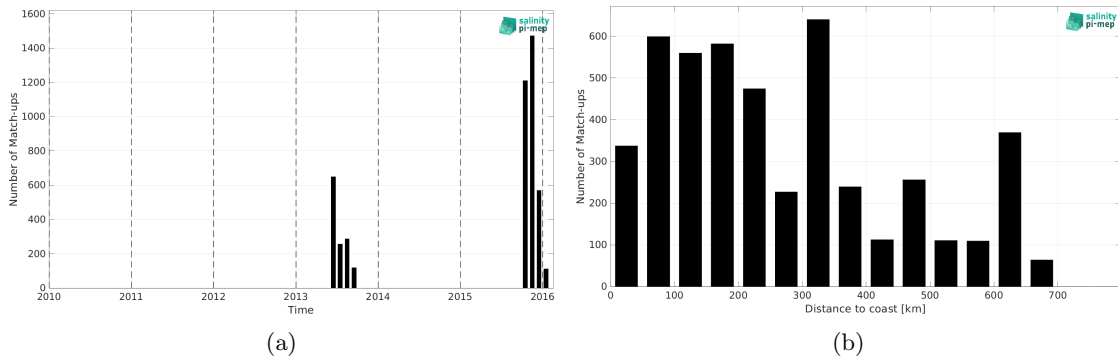
Figure 2: Number of match-ups between Surface drifters and SMOS SSS L3 v335 - 10 Days - 25 km (CATDS-CPDC) SSS as a function of time (a) and as function of the distance to coast (b) over the Ganga and Brahmaputra river plumes Pi-MEP region and for the full satellite product period.
