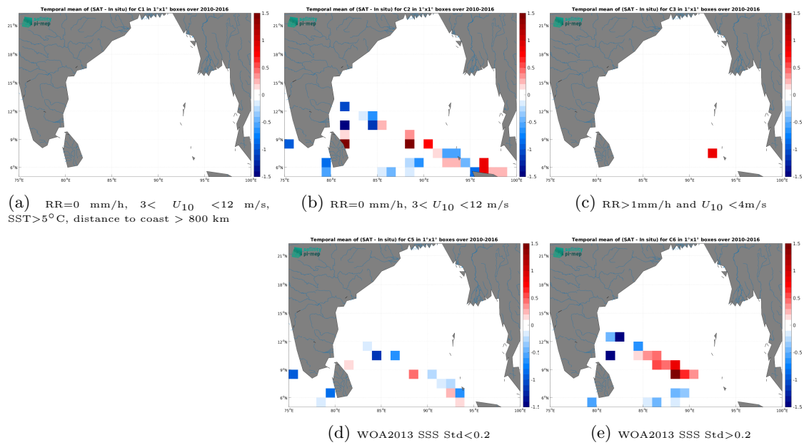
Figure 14: Temporal mean gridded over spatial boxes of size 1^\circ \times 1^\circ of \Delta SSS (SMOS SSS L2Q v333 - 0.25 Deg (CATDS-CPDC) - TSG (LEGOS-DM)) for 5 different subdatasets corresponding to:RR=0 mm/h, 3 < U_{10} < 12 m/s, SST >5^\circ C, distance to coast > 800 km (a), RR=0 mm/h, 3 < U_{10} < 12 m/s (b), RR >1 mm/h and U_{10} < 4 m/s (c), WOA2013 SSS Std <0.2 (d), WOA2013 SSS Std >0.2 (e).
