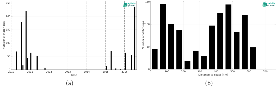
Figure 2: Number of match-ups between TSG (LEGOS-DM) and SMOS SSS L2Q v333 - 0.25 Deg (CATDS-CPDC) SSS as a function of time (a) and as function of the distance to coast (b) over the Ganga and Brahmaputra river plumes Pi-MEP region and for the full satellite product period.
