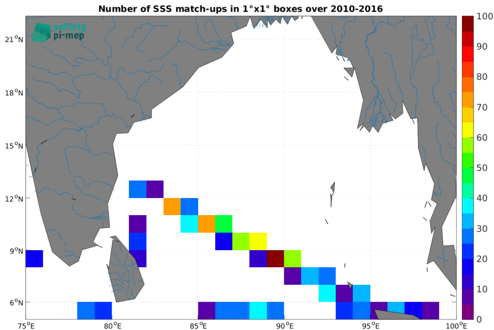
Figure 5: Number of SSS match-ups between TSG (LEGOS-DM) SSS and the SMOS SSS L2Q v333 - 0.25 Deg (CATDS-CPDC) SSS product for the Ganga and Brahmaputra river plumes Pi-MEP region over 1^\circ \times 1^\circ boxes and for the full satellite product period.
