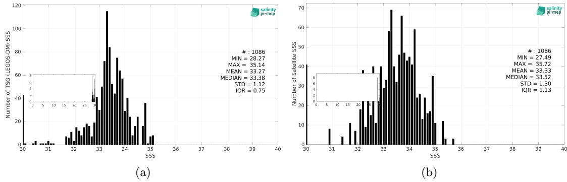
Figure 3: Histograms of SSS from TSG (LEGOS-DM) (a) and SMOS SSS L2Q v333 - 0.25 Deg (CATDS-CPDC) (b) considering all match-up pairs per bins of 0.1 over the Ganga and Brahmaputra river plumes Pi-MEP region and for the full satellite product period.
