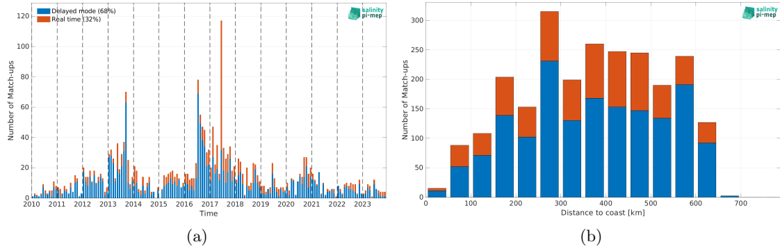
Figure 2: Number of match-ups between Argo and SMOS SSS L2Q v333 - 0.25 Deg (CATDS-CPDC) SSS as a function of time (a) and as function of the distance to coast (b) over the Ganga and Brahmaputra river plumes Pi-MEP region and for the full satellite product period.
