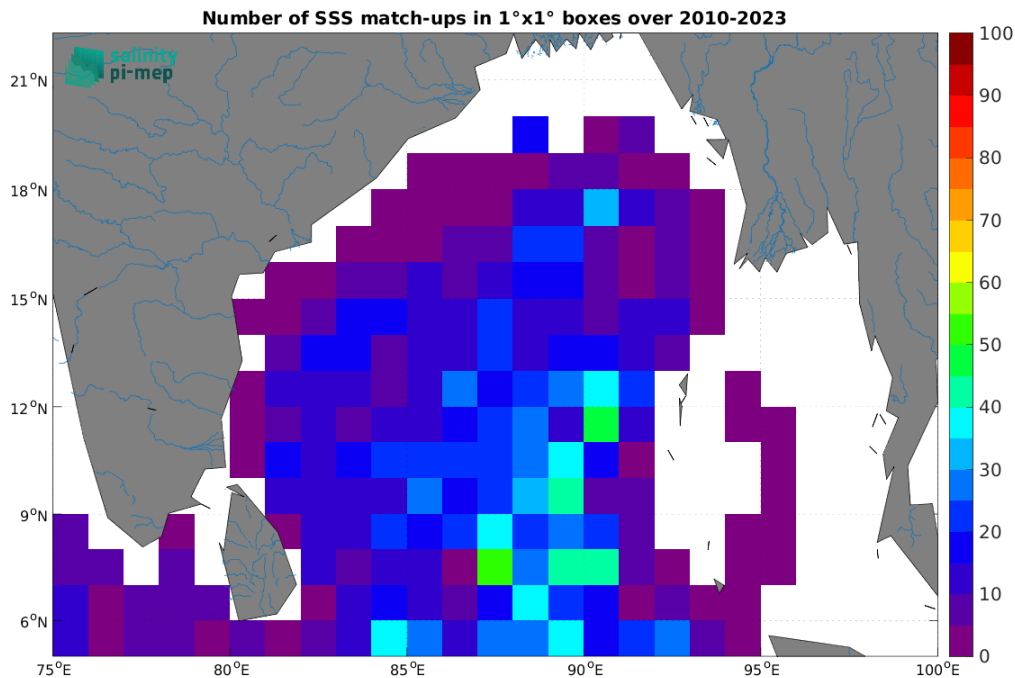
Figure 5: Number of SSS match-ups between Argo SSS and the SMOS SSS L2Q v333 - 0.25 Deg (CATDS-CPDC) SSS product for the Ganga and Brahmaputra river plumes Pi-MEP region over 1^\circ \times 1^\circ boxes and for the full satellite product period.
