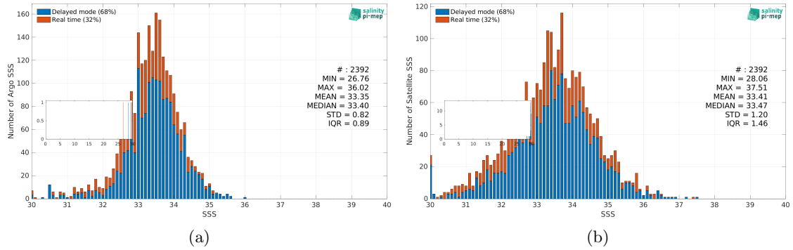
Figure 3: Histograms of SSS from Argo (a) and SMOS SSS L2Q v333 - 0.25 Deg (CATDS-CPDC) (b) considering all match-up pairs per bins of 0.1 over the Ganga and Brahmaputra river plumes Pi-MEP region and for the full satellite product period.
