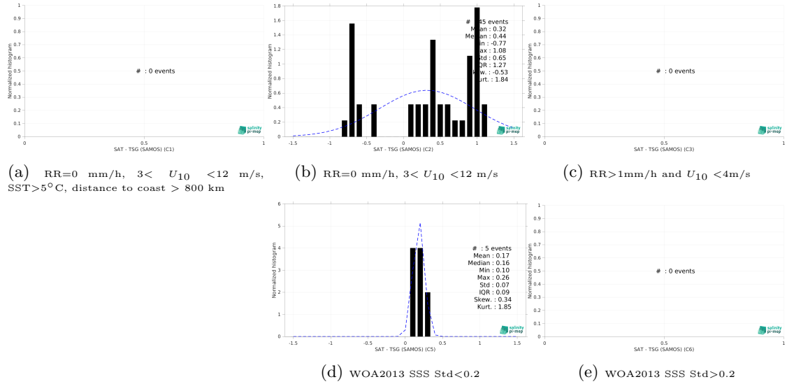
Figure 15: Normalized histogram of \Delta SSS (SMOS SSS L3 v332 - 9 Days (CATDS-CPDC) - TSG (SAMOS)) for 5 different subdatasets corresponding to: RR=0 mm/h, 3 < U_{10} < 12 m/s, SST > 5^\circ\text{C} , distance to coast > 800 km (a), RR=0 mm/h, 3 < U_{10} < 12 m/s (b), RR > 1 mm/h and U_{10} < 4 m/s (c), WOA2013 SSS Std < 0.2 (d), WOA2013 SSS Std > 0.2 (e).
